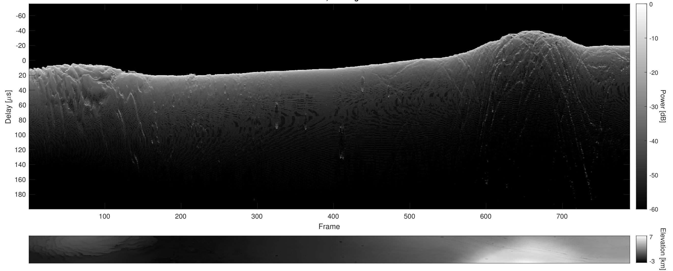
Orbit 15806, Cluttergram
