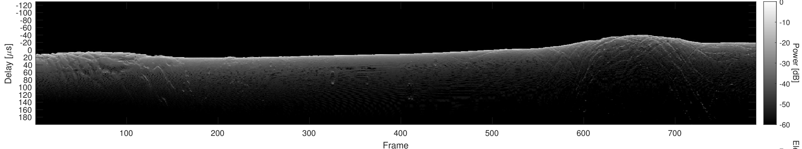
Orbit 15806, Cluttergram
