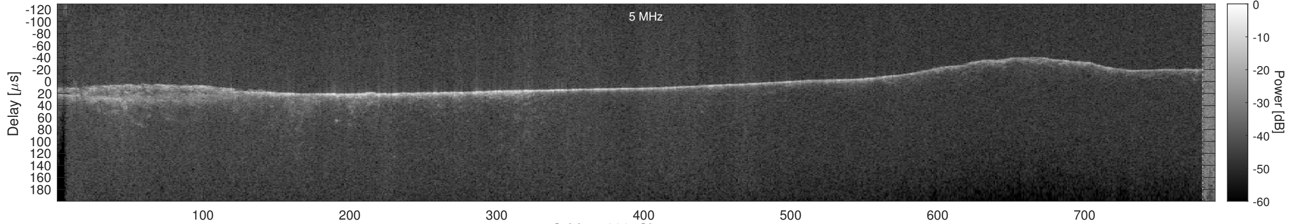
Orbit 15806, Cluttergram
