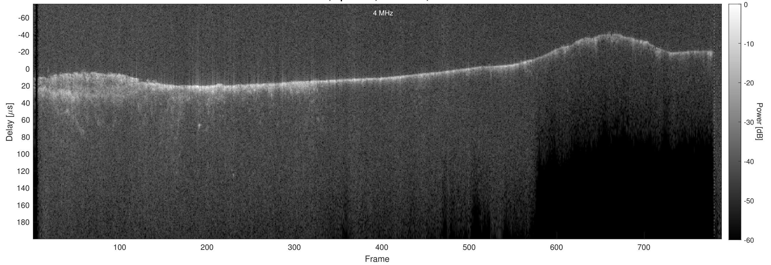
Orbit 15806, Optimized, No Window, Channel 2
