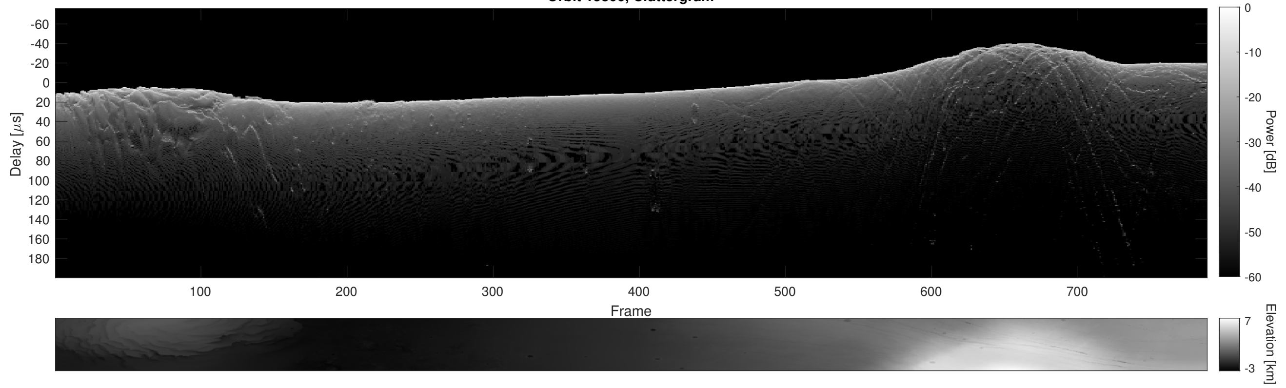
Orbit 15806, Cluttergram
