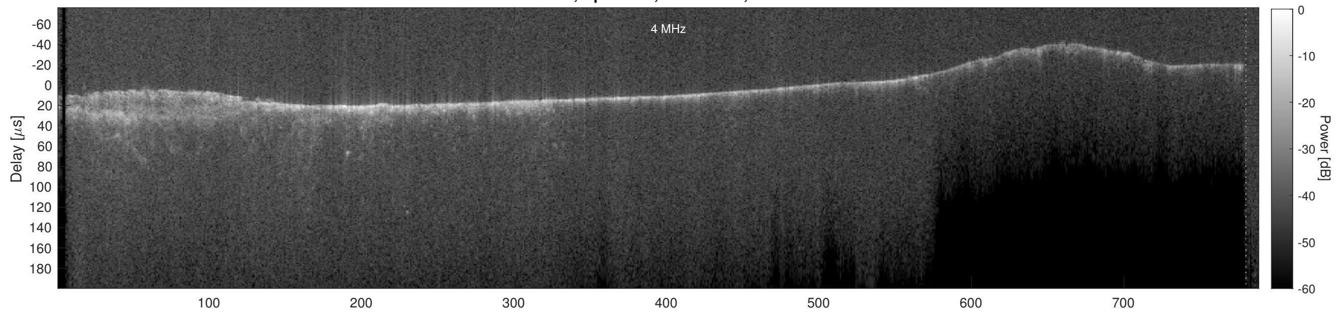
Orbit 15806, Cluttergram
