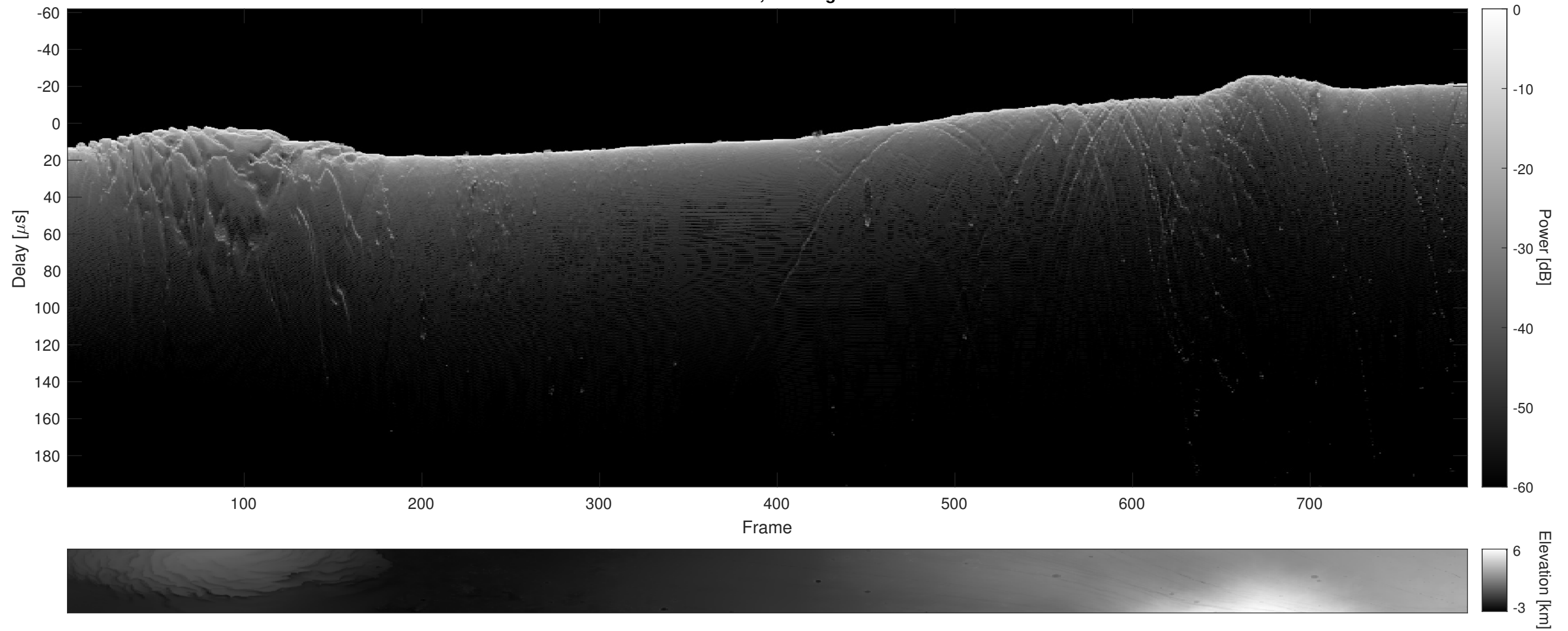
Orbit 15813, Cluttergram
