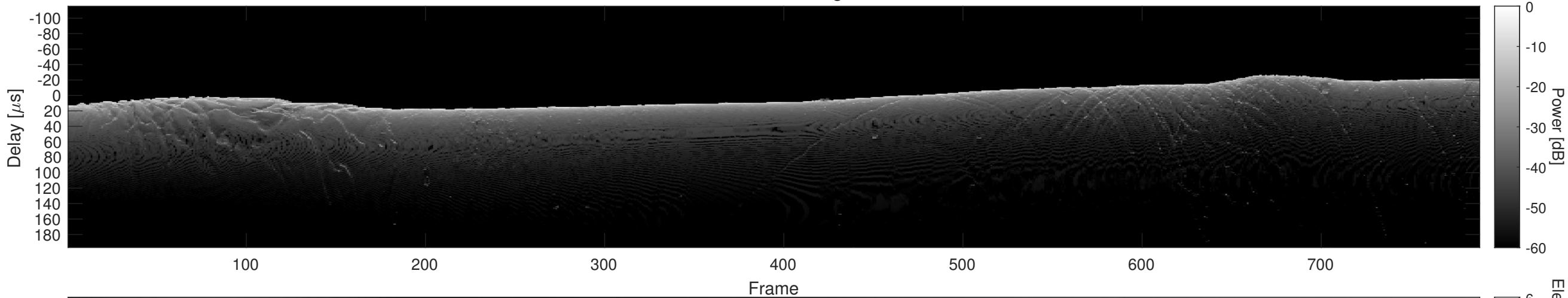
Orbit 15813, Cluttergram
