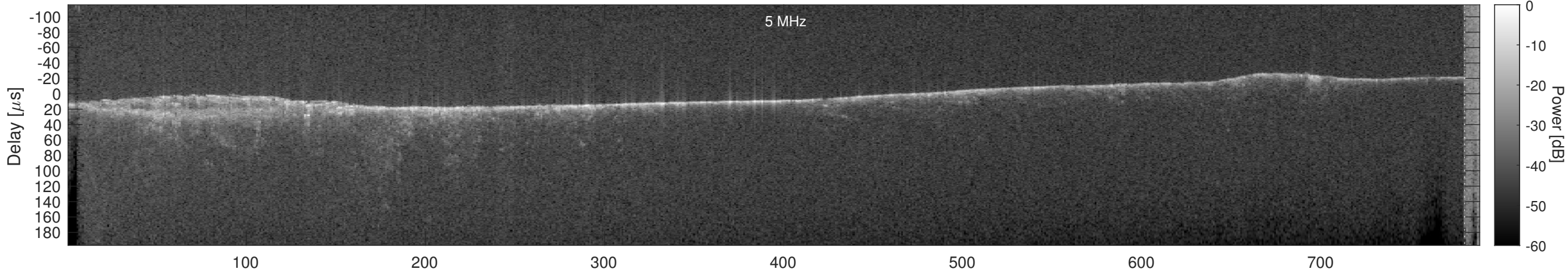
Orbit 15813, Cluttergram
