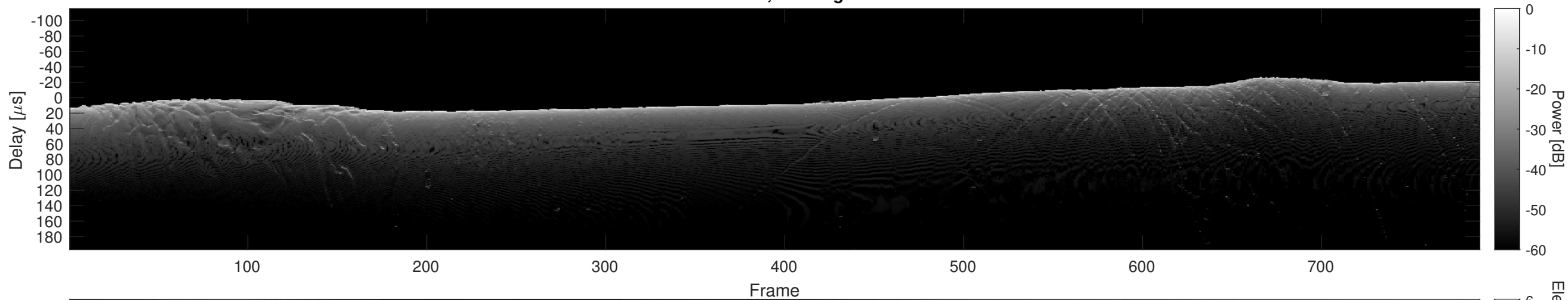
Orbit 15813, Cluttergram
