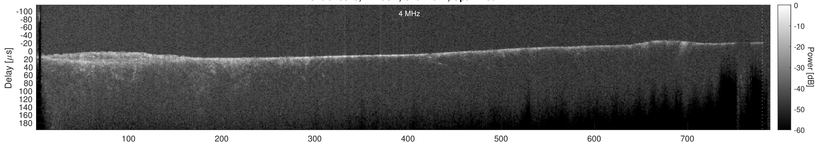
Orbit 15813, Cluttergram
