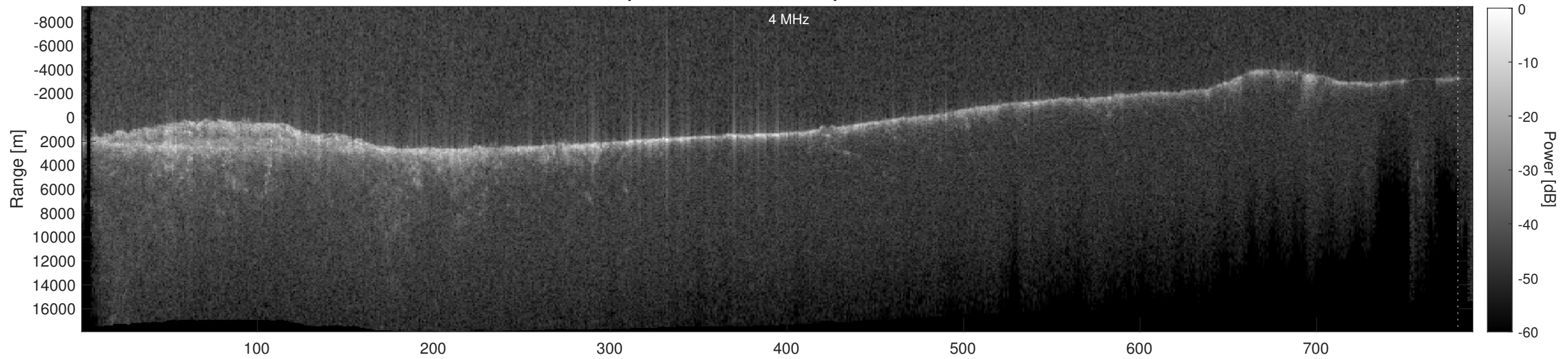
Orbit 15813, Depth-Corrected Cluttergram
