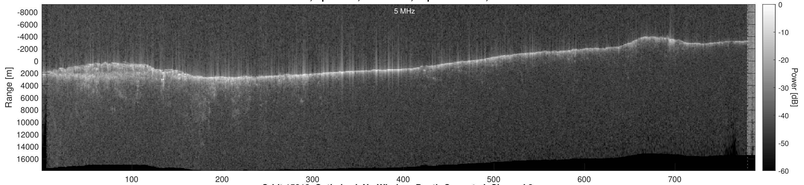
Orbit 15813, Optimized, No Window, Depth-Corrected, Channel 2
