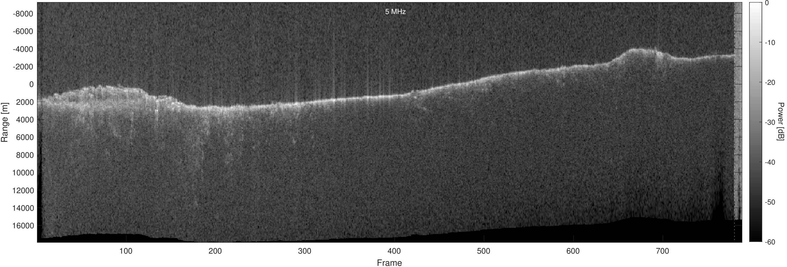
Orbit 15813, Optimized, Window, Depth-Corrected, Channel 2
