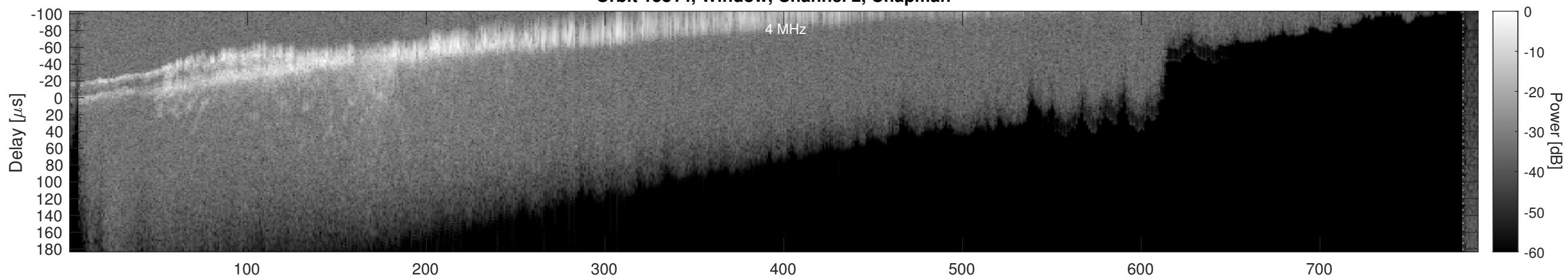
Orbit 15814, Window, Channel 2, Optimized
