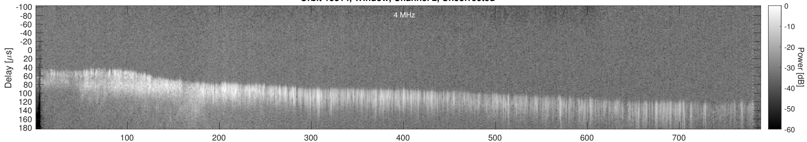
Orbit 15814, Window, Channel 2, Chapman
