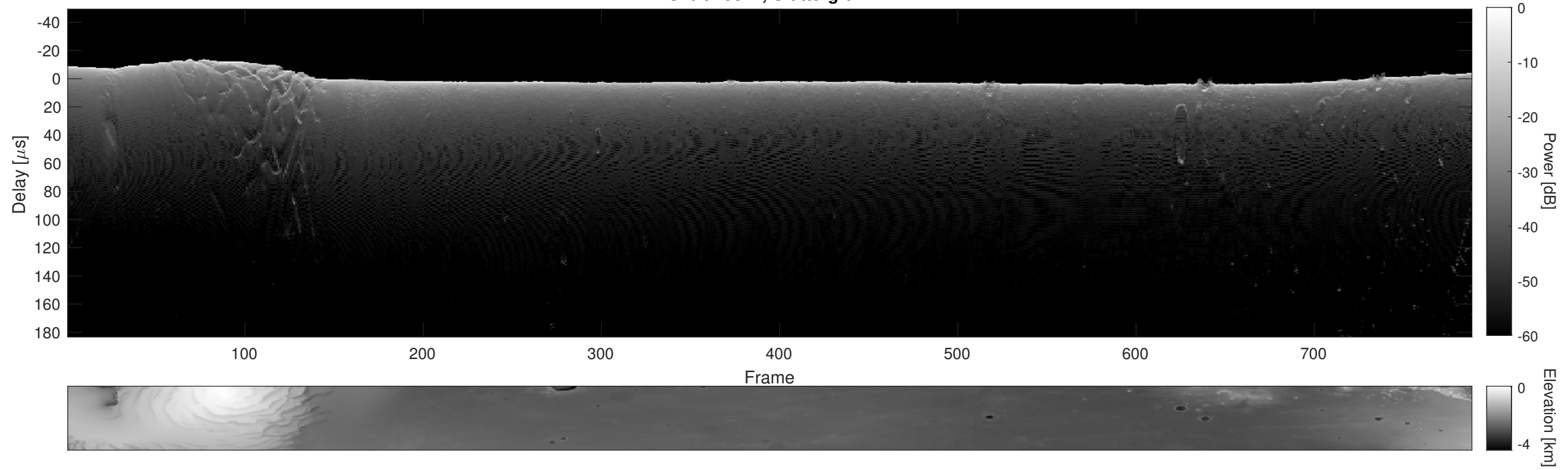
Orbit 15814, Cluttergram
