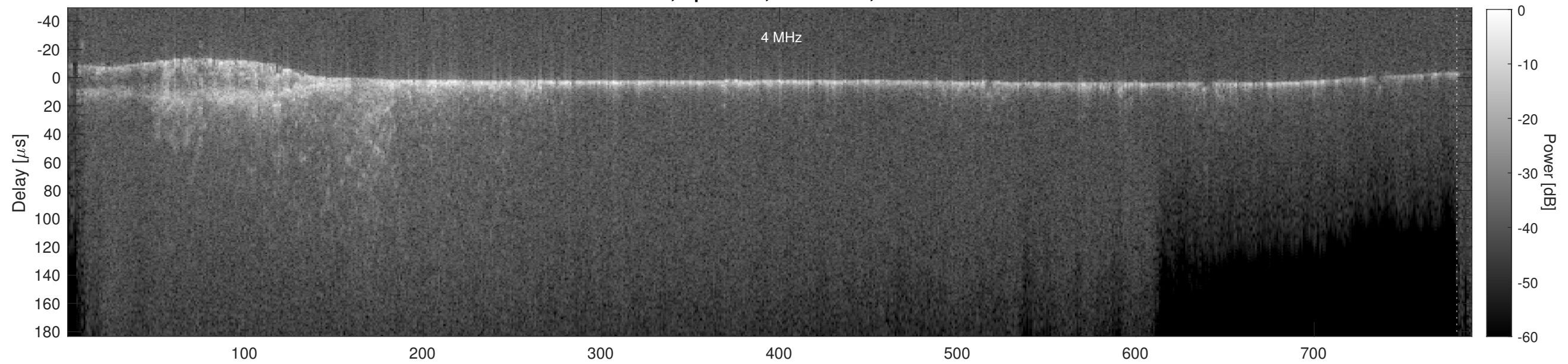
Orbit 15814, Cluttergram
