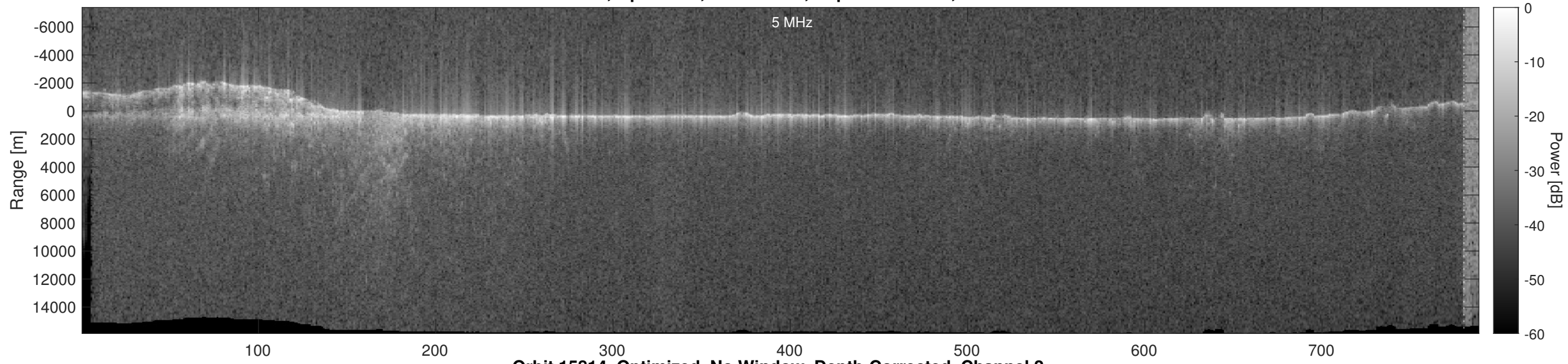
Orbit 15814, Optimized, No Window, Depth-Corrected, Channel 2
