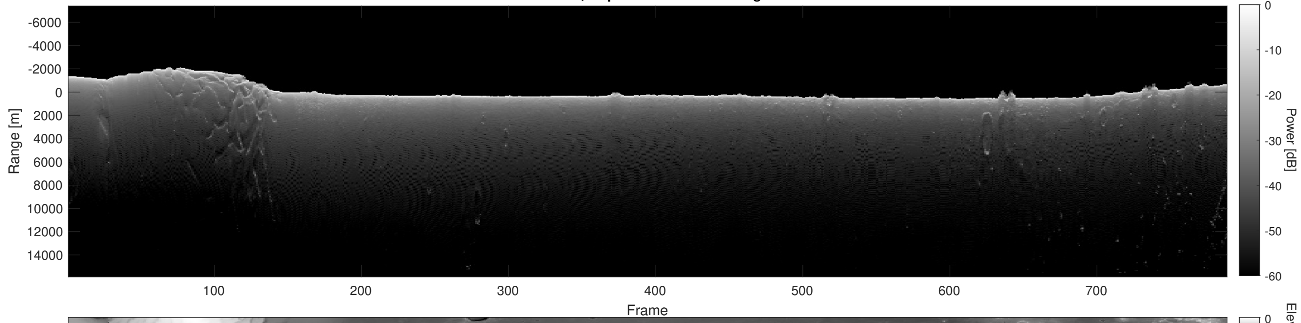
Orbit 15814, Depth-Corrected Cluttergram
