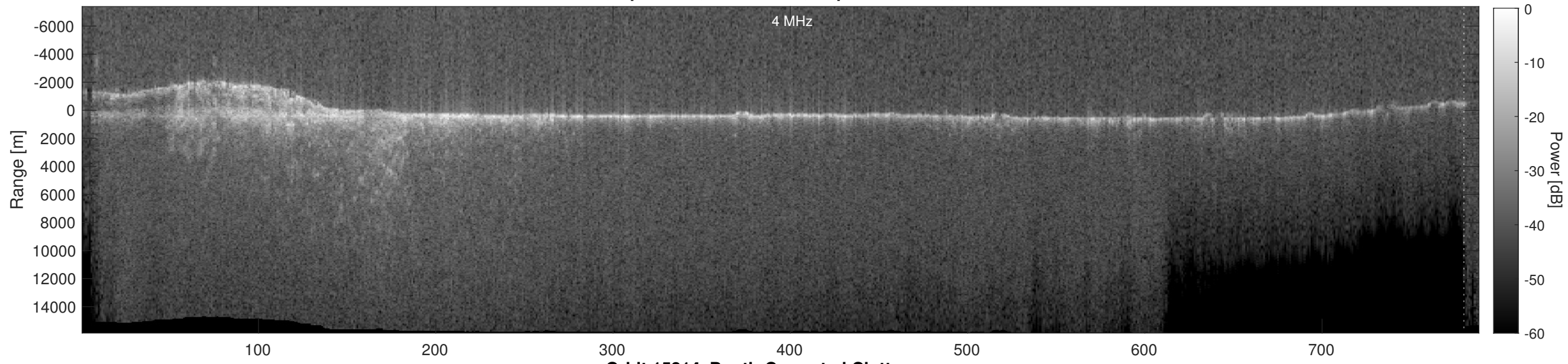
Orbit 15814, Depth-Corrected Cluttergram
