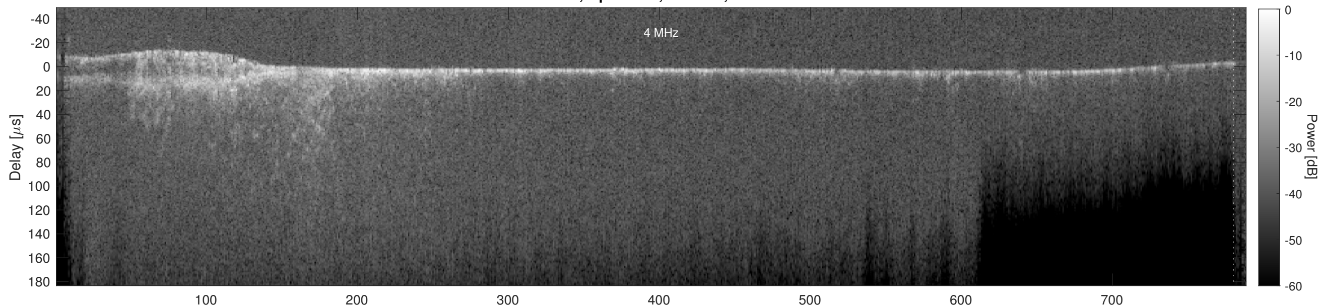
Orbit 15814, Cluttergram
