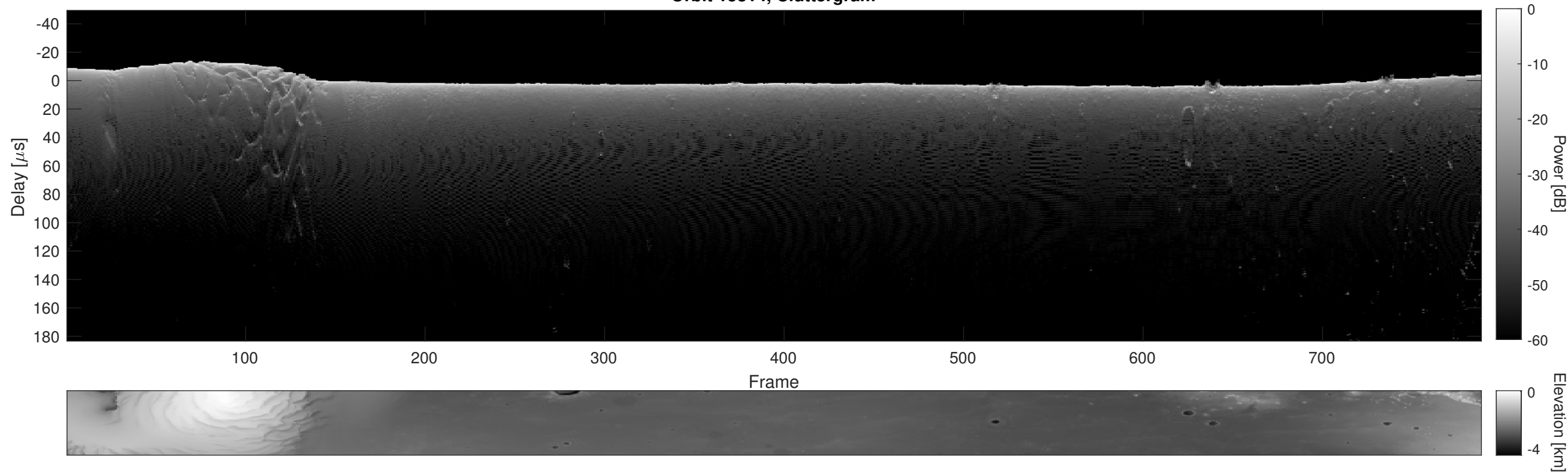
Orbit 15814, Cluttergram
