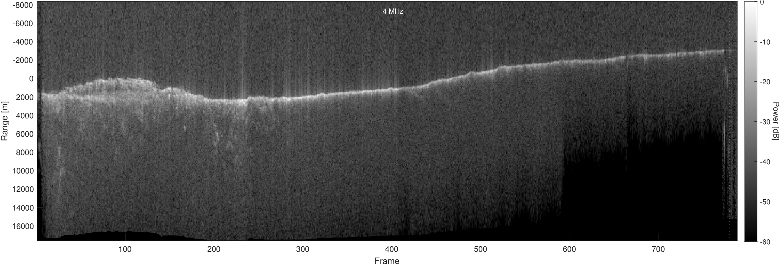
Orbit 15820, Optimized, No Window, Depth-Corrected, Channel 2
