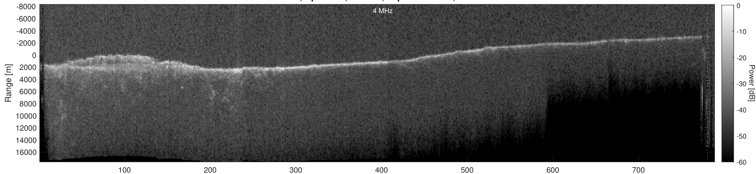
Orbit 15820, Depth-Corrected Cluttergram
