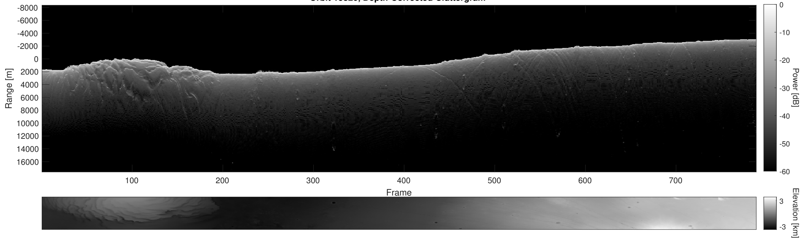
Orbit 15820, Depth-Corrected Cluttergram
