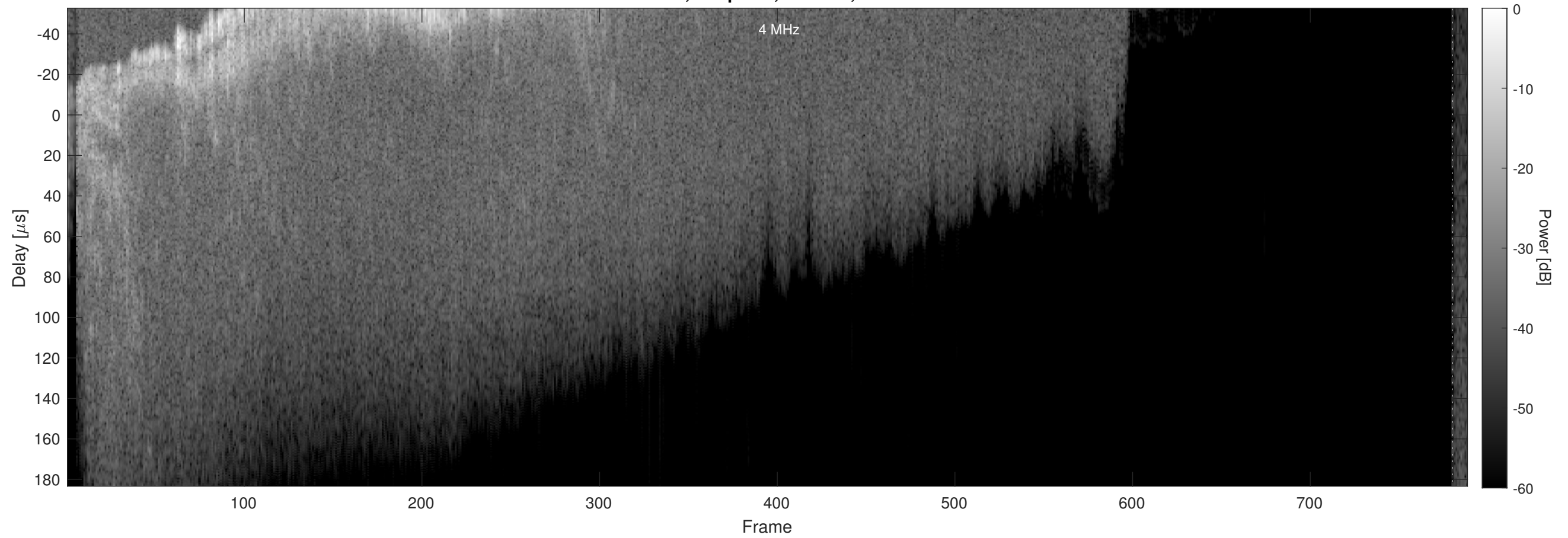
Orbit 15823, Chapman, Window, Channel 2
