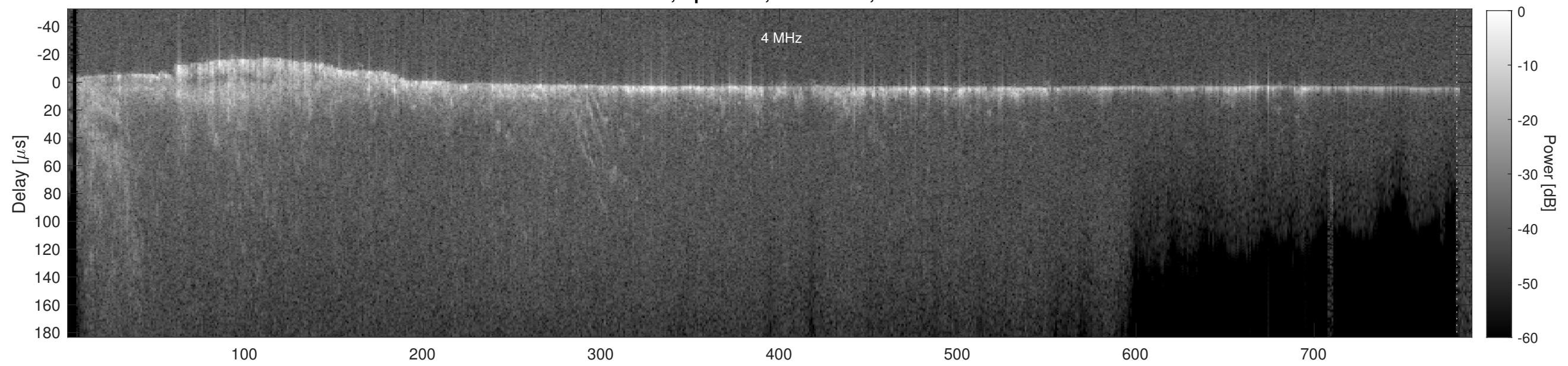
Orbit 15823, Cluttergram
