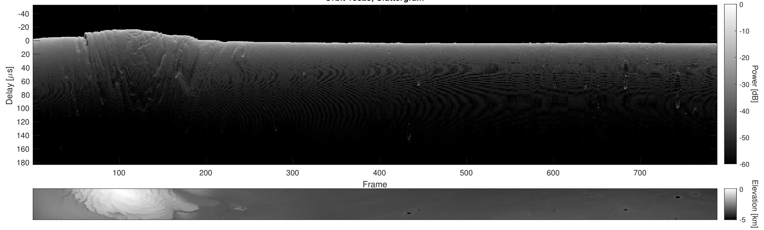
Orbit 15823, Cluttergram
