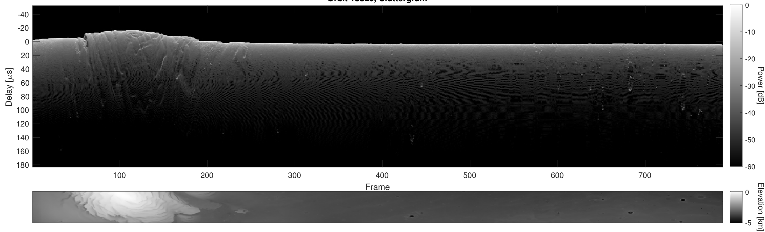
Orbit 15823, Cluttergram
