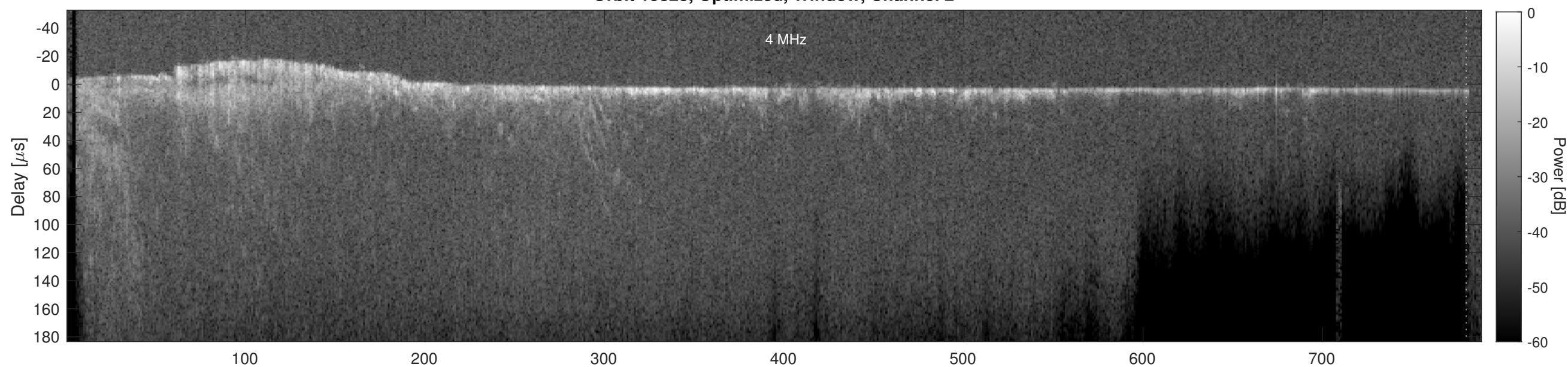
Orbit 15823, Cluttergram
