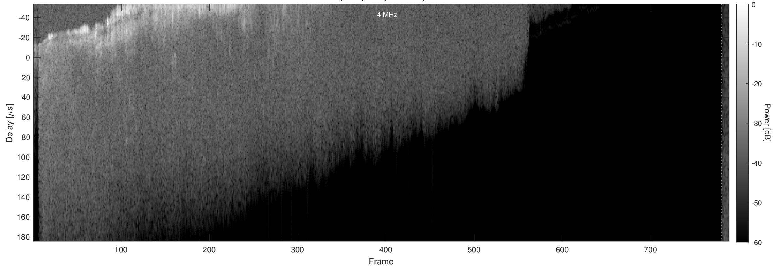
Orbit 15830, Chapman, Window, Channel 2
