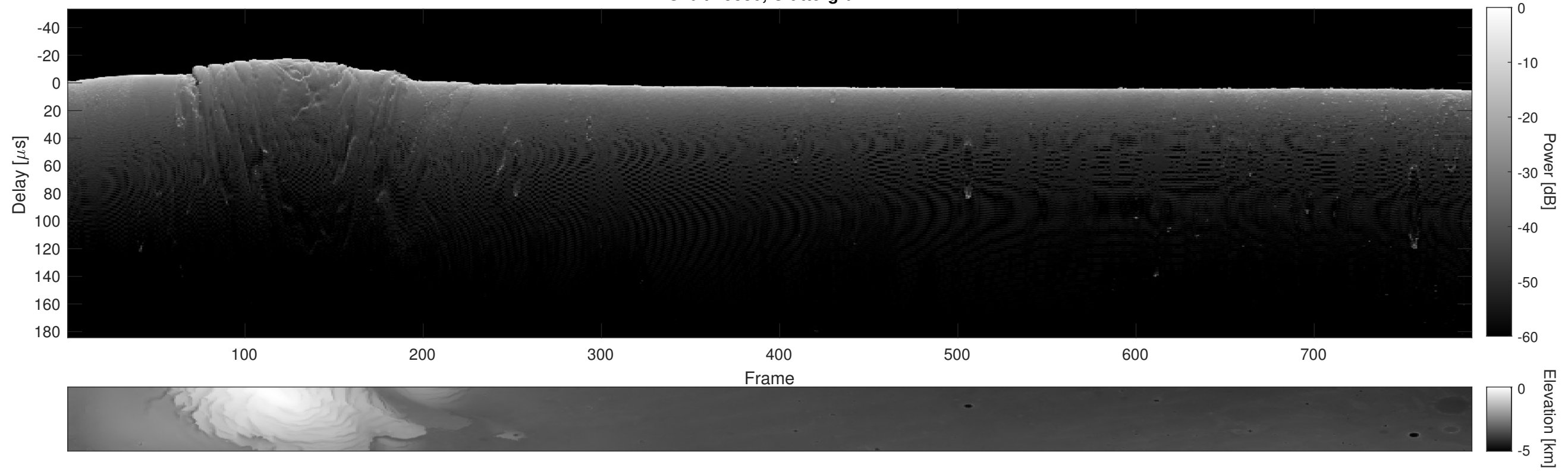
Orbit 15830, Cluttergram
