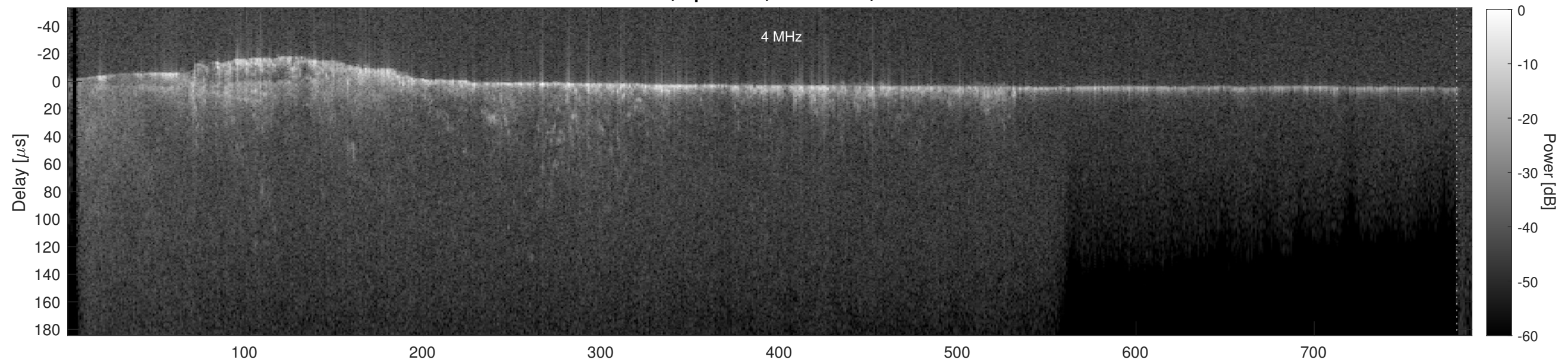
Orbit 15830, Cluttergram
