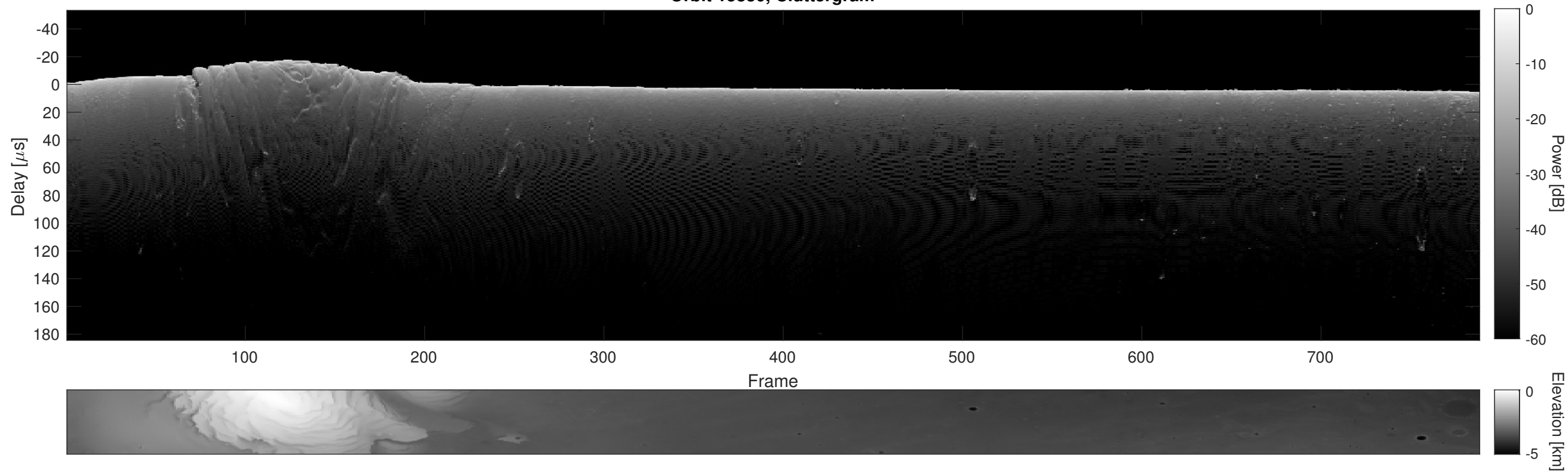
Orbit 15830, Cluttergram
