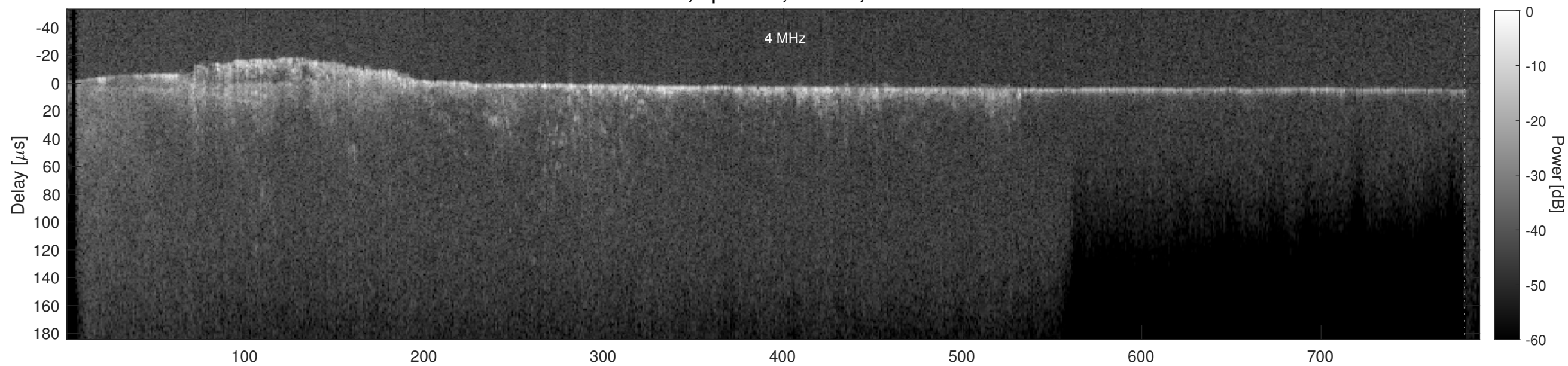
Orbit 15830, Cluttergram
