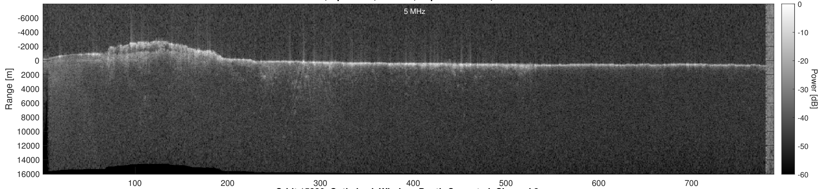
Orbit 15830, Optimized, Window, Depth-Corrected, Channel 2
