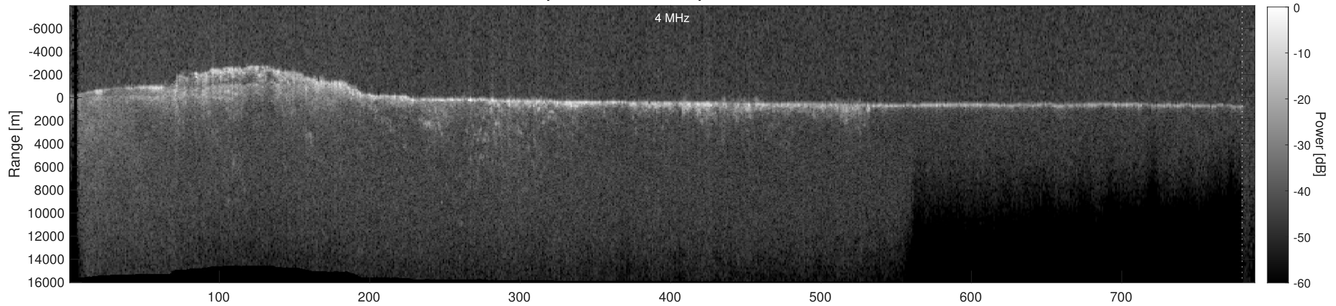
Orbit 15830, Depth-Corrected Cluttergram
