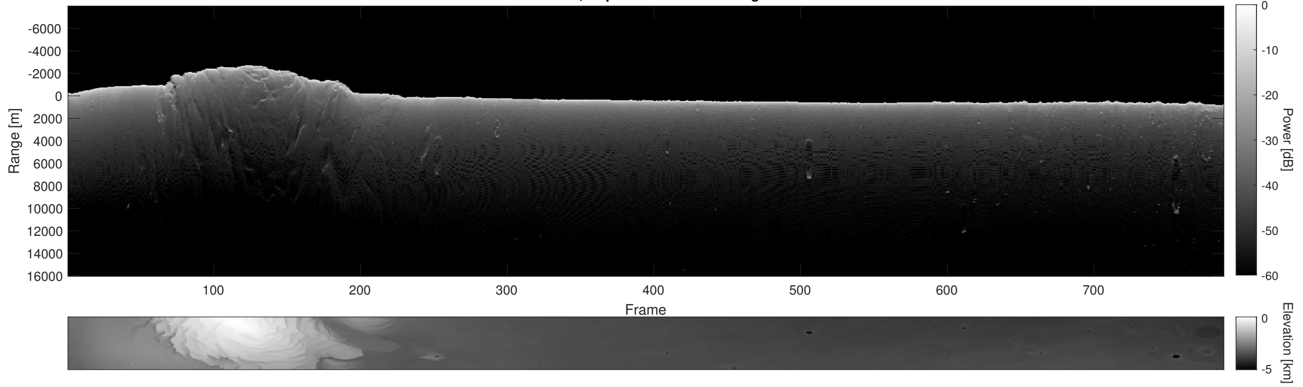
Orbit 15830, Depth-Corrected Cluttergram
