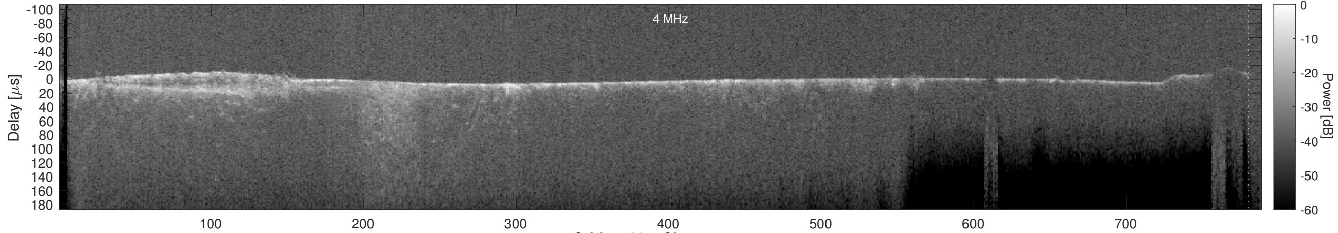
Orbit 15831, Cluttergram
