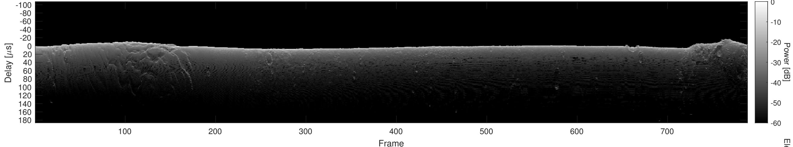
Orbit 15831, Cluttergram
