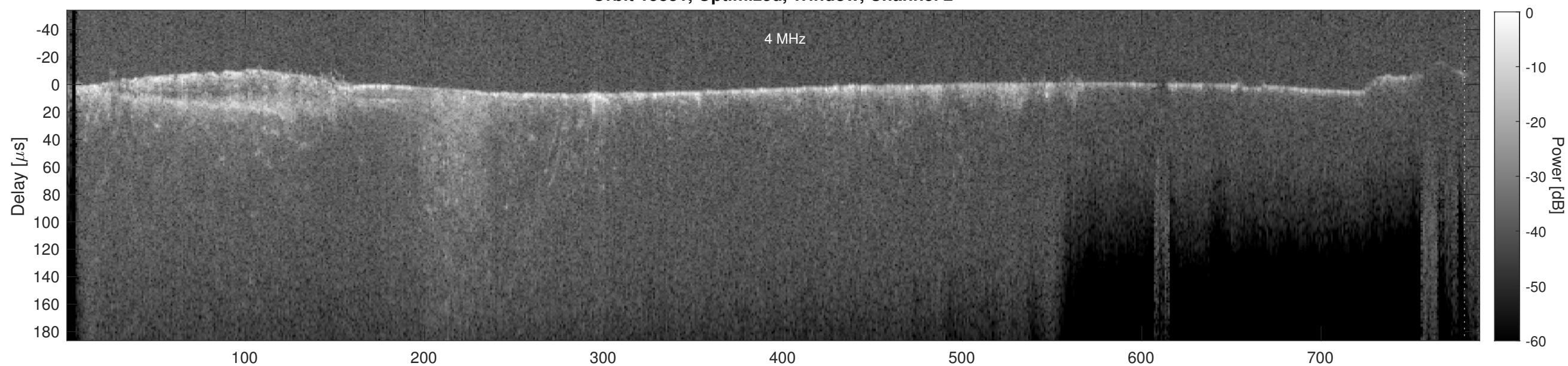
Orbit 15831, Cluttergram
