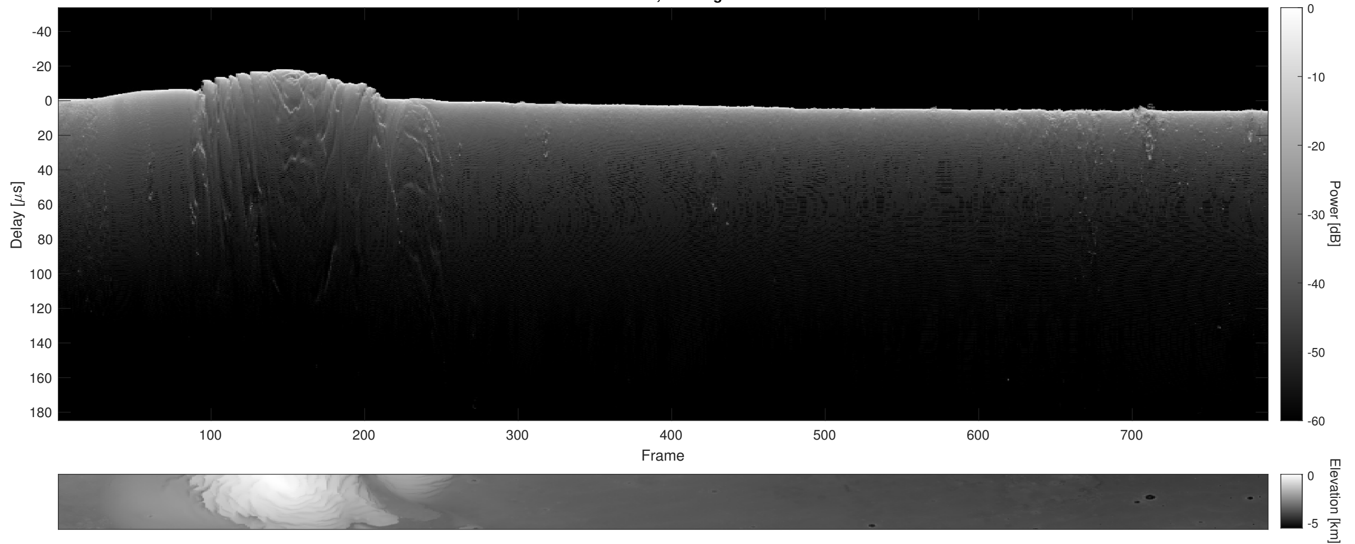
Orbit 15844, Cluttergram
