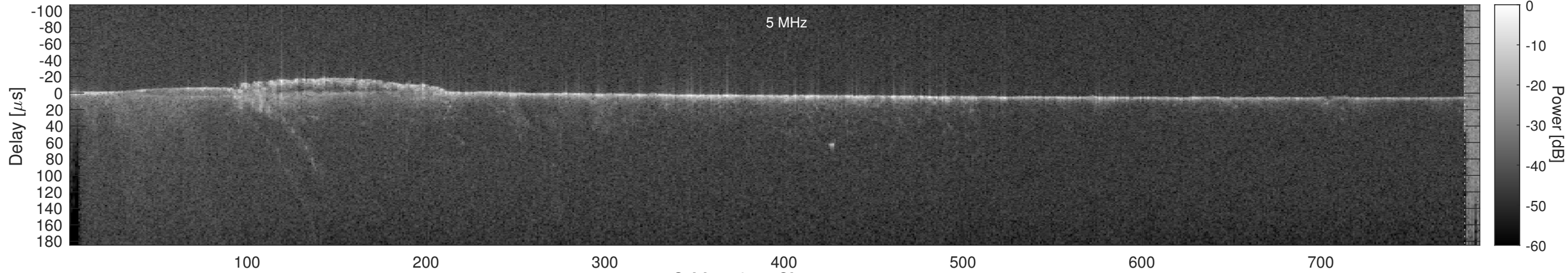
Orbit 15844, Cluttergram
