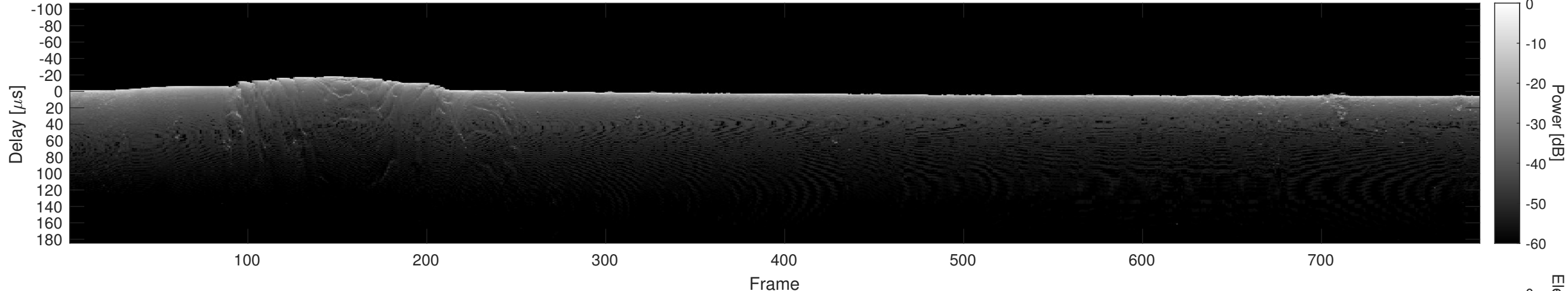
Orbit 15844, Cluttergram
