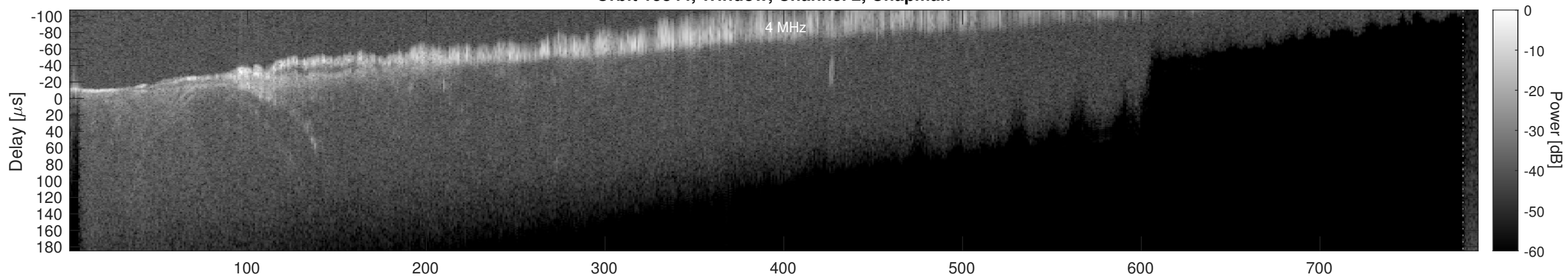
Orbit 15844, Window, Channel 2, Optimized
