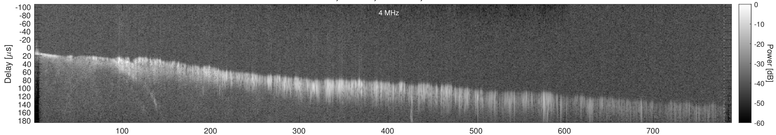
Orbit 15844, Window, Channel 2, Chapman
