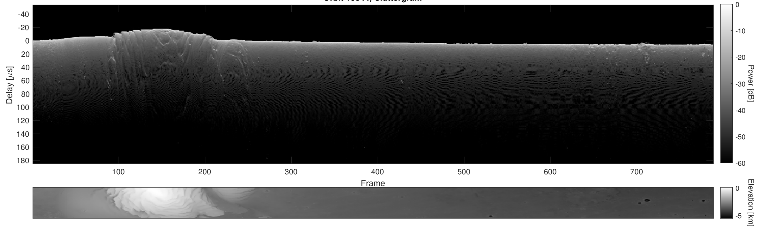
Orbit 15844, Cluttergram
