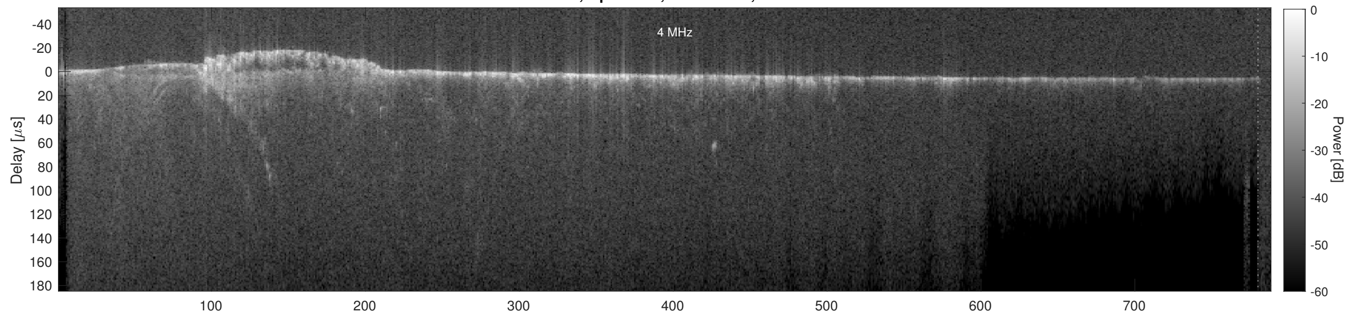
Orbit 15844, Cluttergram
