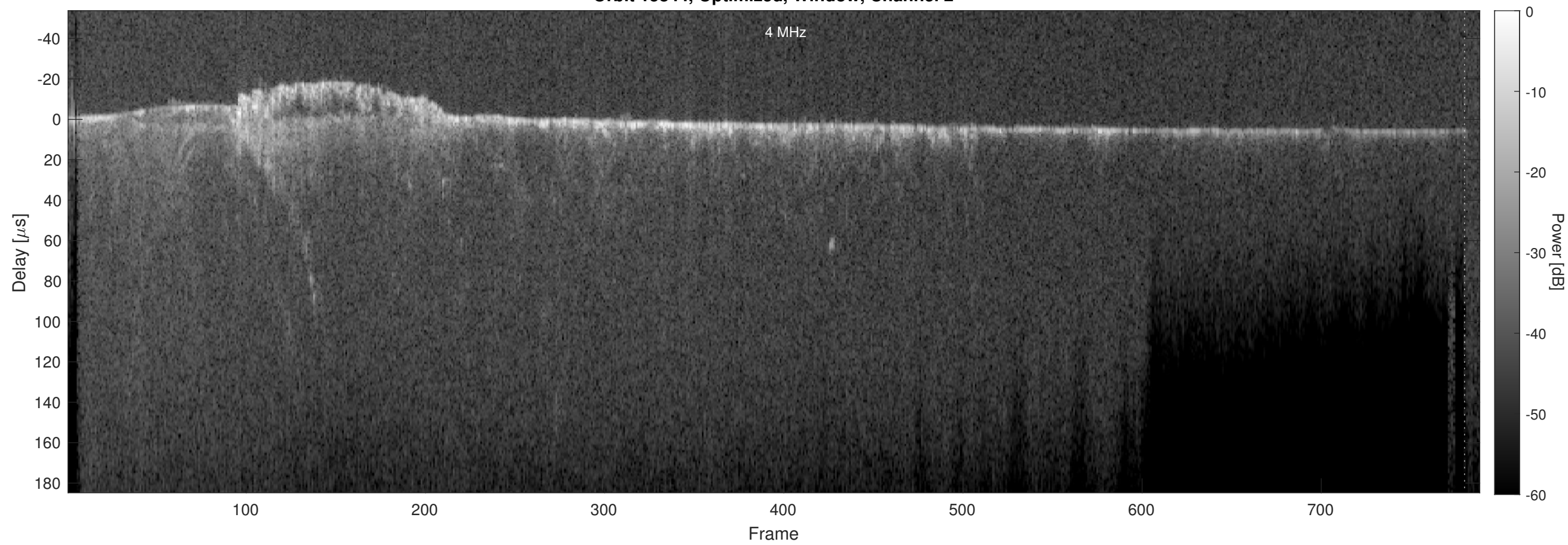
Orbit 15844, Optimized, Window, Channel 2
