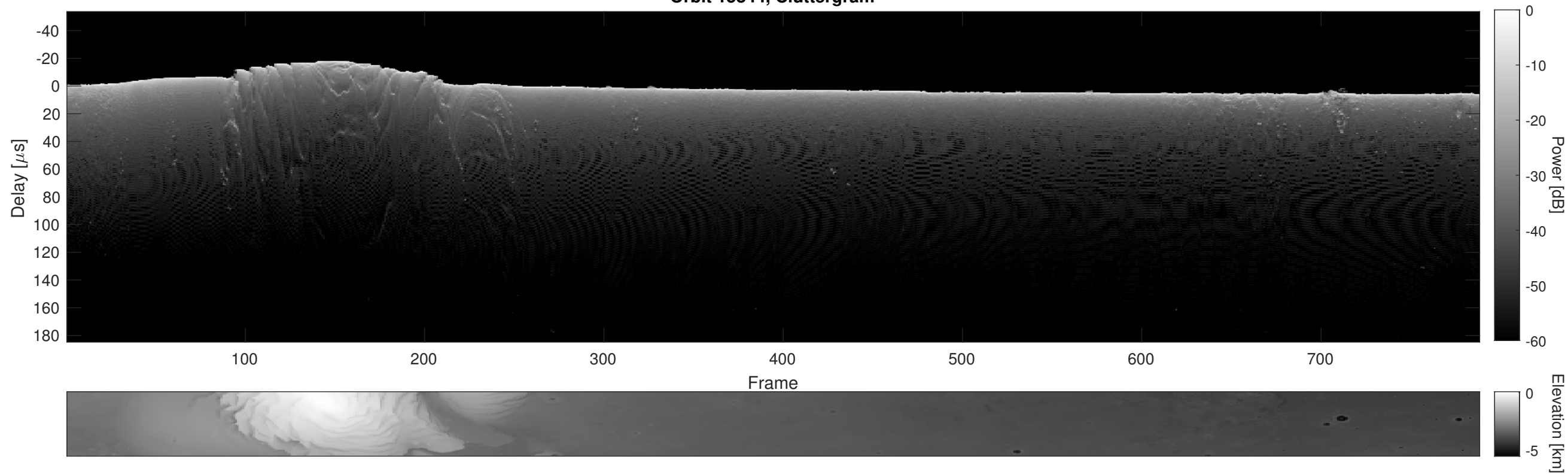
Orbit 15844, Cluttergram
