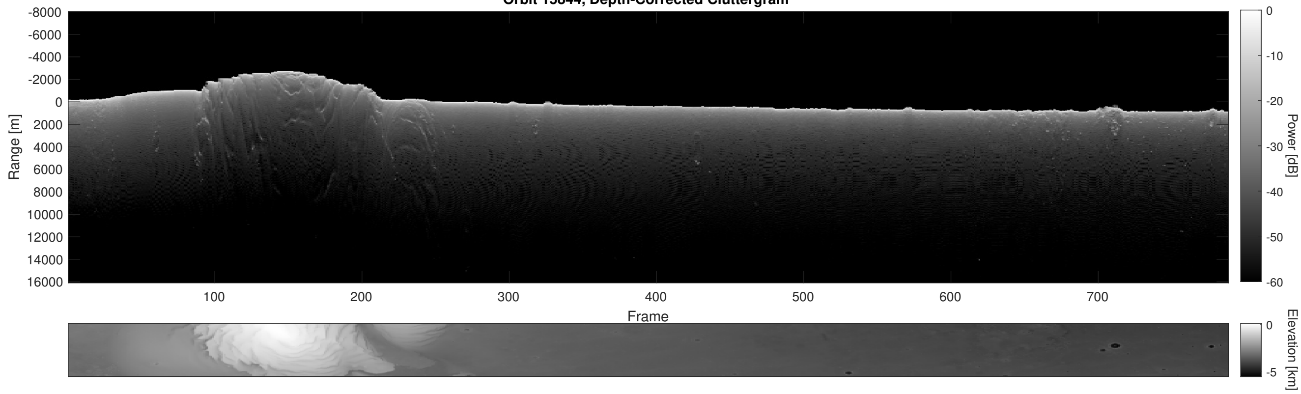
Orbit 15844, Depth-Corrected Cluttergram
