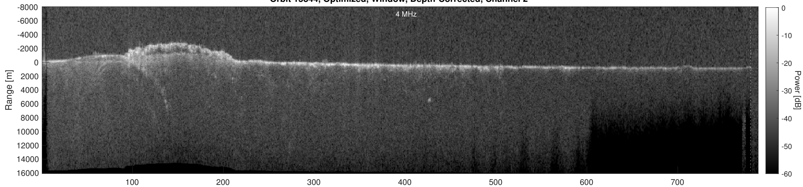
Orbit 15844, Depth-Corrected Cluttergram
