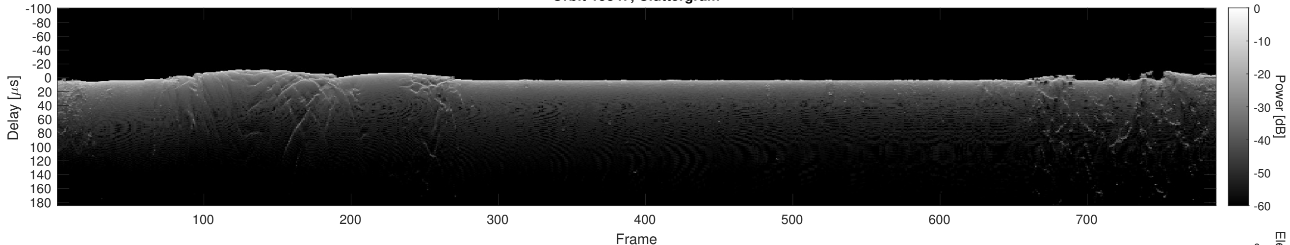
Orbit 15847, Cluttergram
