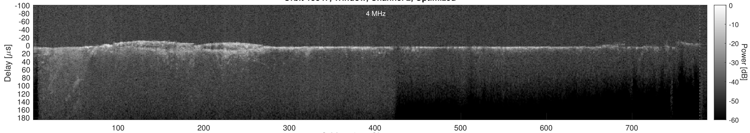
Orbit 15847, Cluttergram
