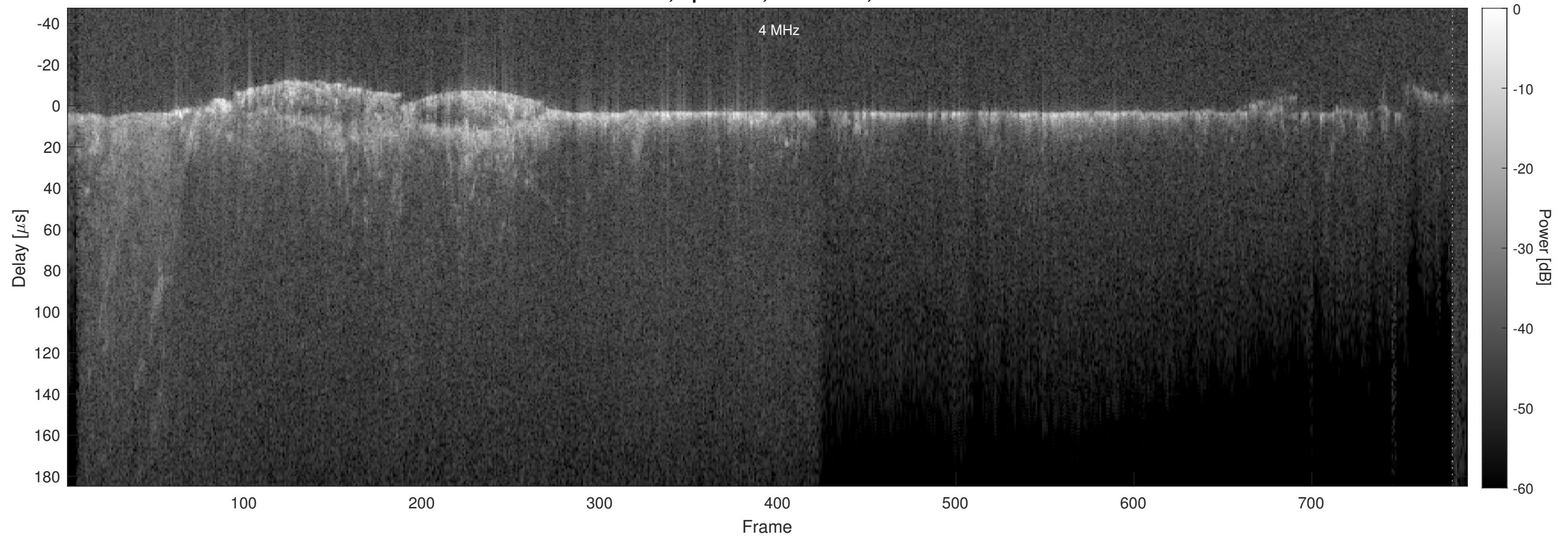
Orbit 15847, Optimized, No Window, Channel 2
