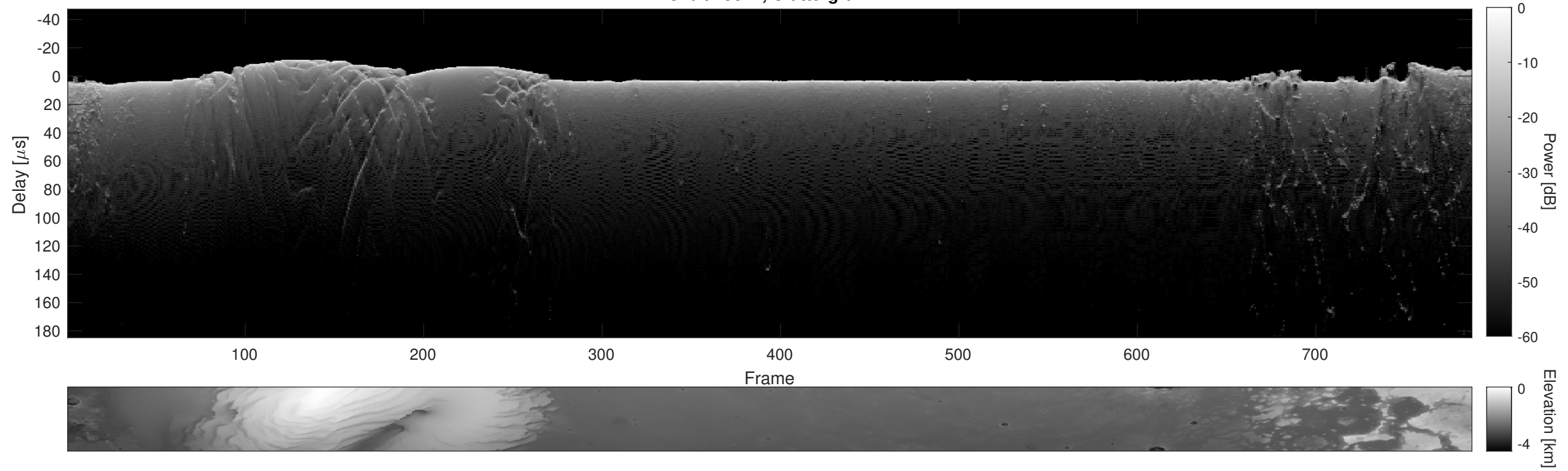
Orbit 15847, Cluttergram
