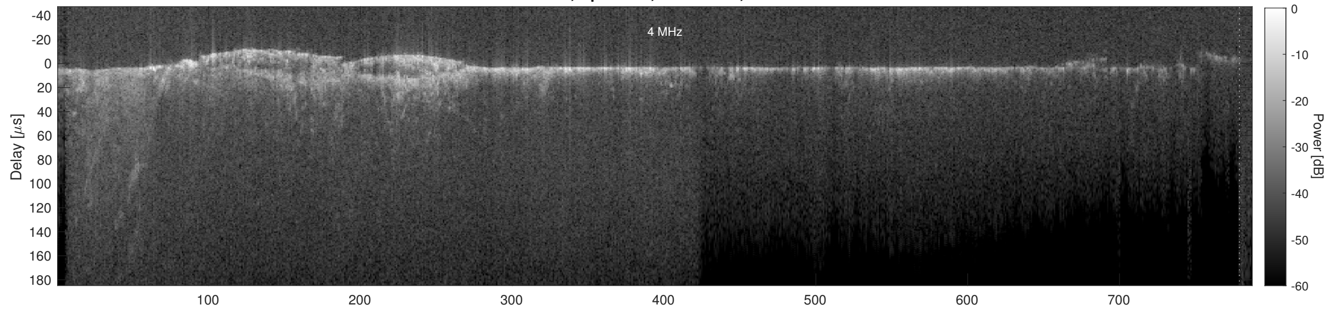
Orbit 15847, Cluttergram
