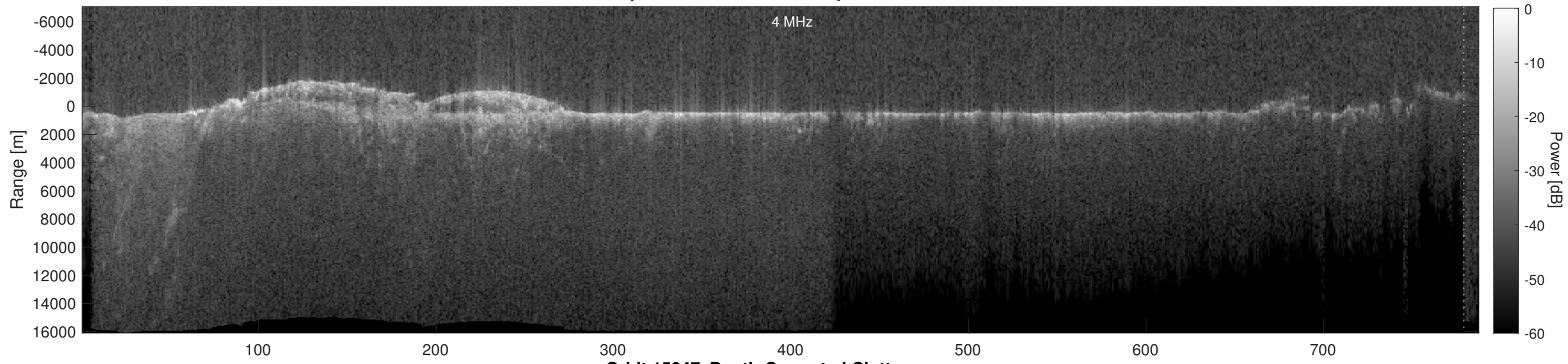
Orbit 15847, Depth-Corrected Cluttergram
