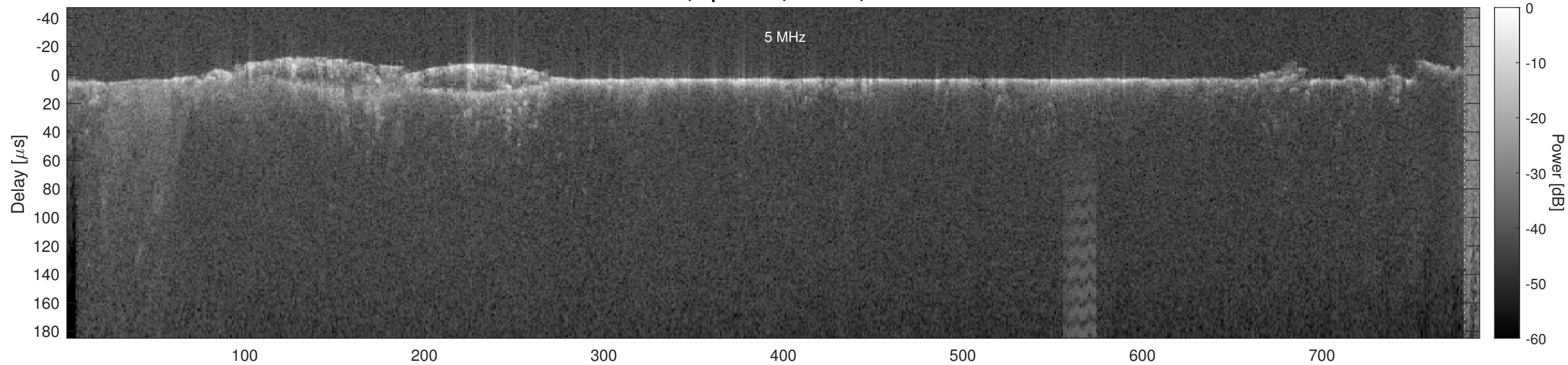
Orbit 15847, Optimized, Window, Channel 2
