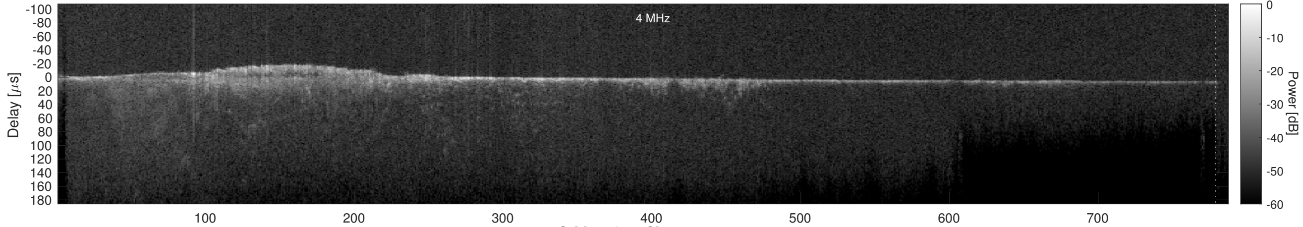
Orbit 15851, Cluttergram
