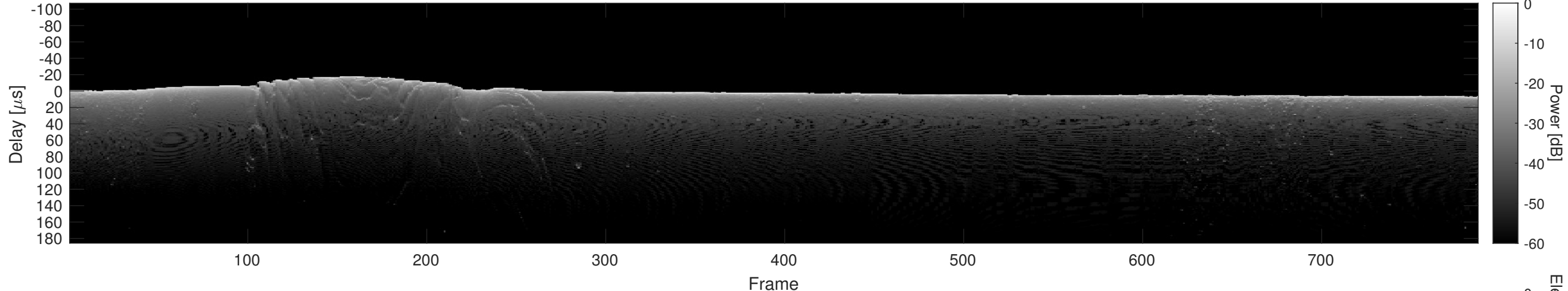
Orbit 15851, Cluttergram
