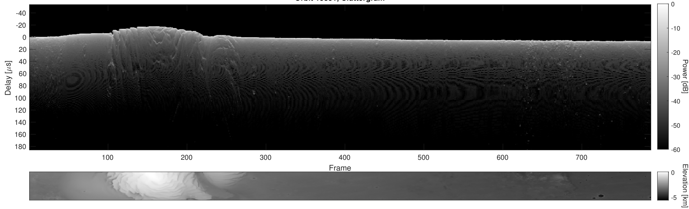
Orbit 15851, Cluttergram
