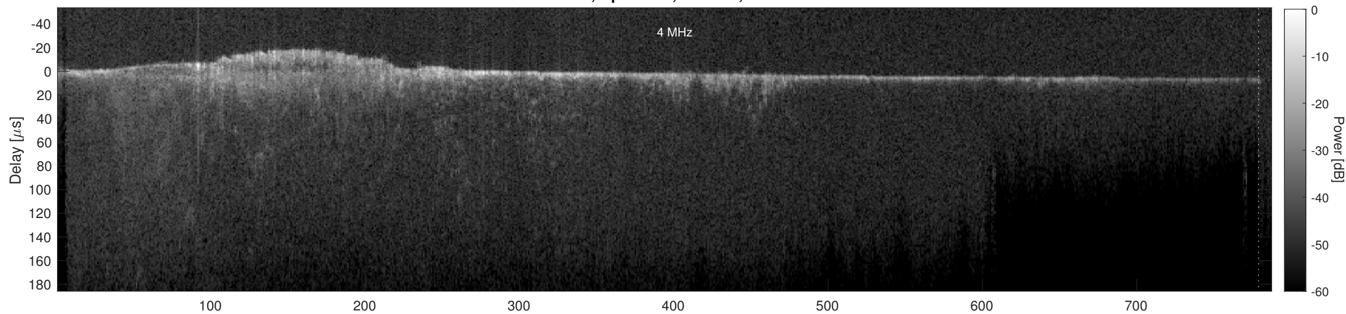
Orbit 15851, Cluttergram
