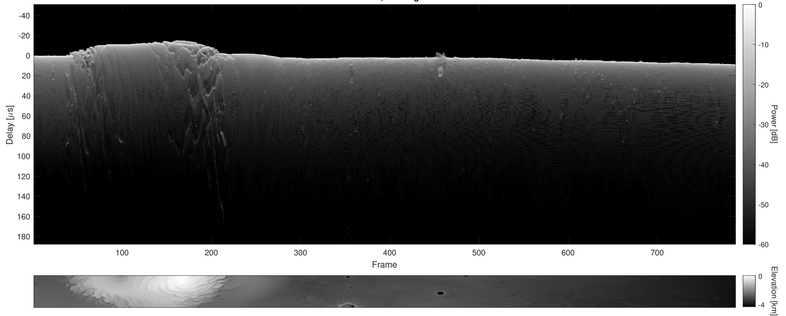
Orbit 15856, Cluttergram
