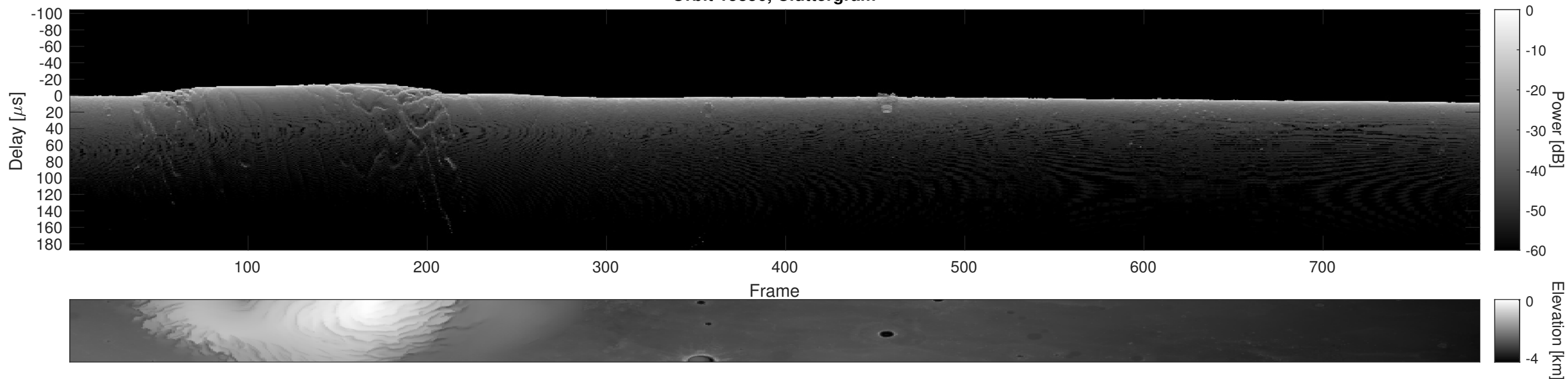
Orbit 15856, Cluttergram
