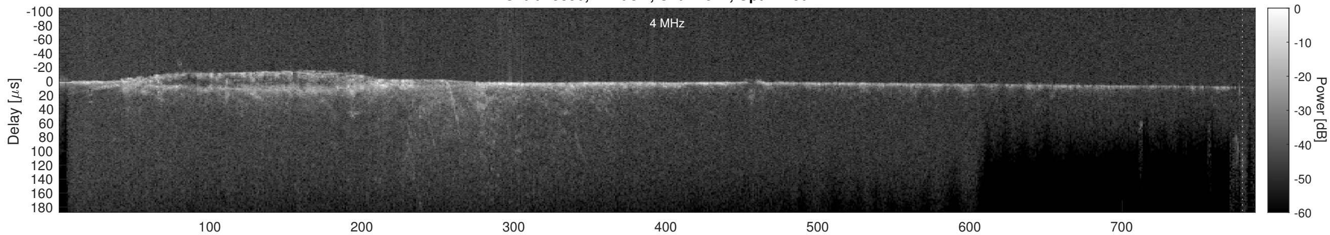
Orbit 15856, Cluttergram
