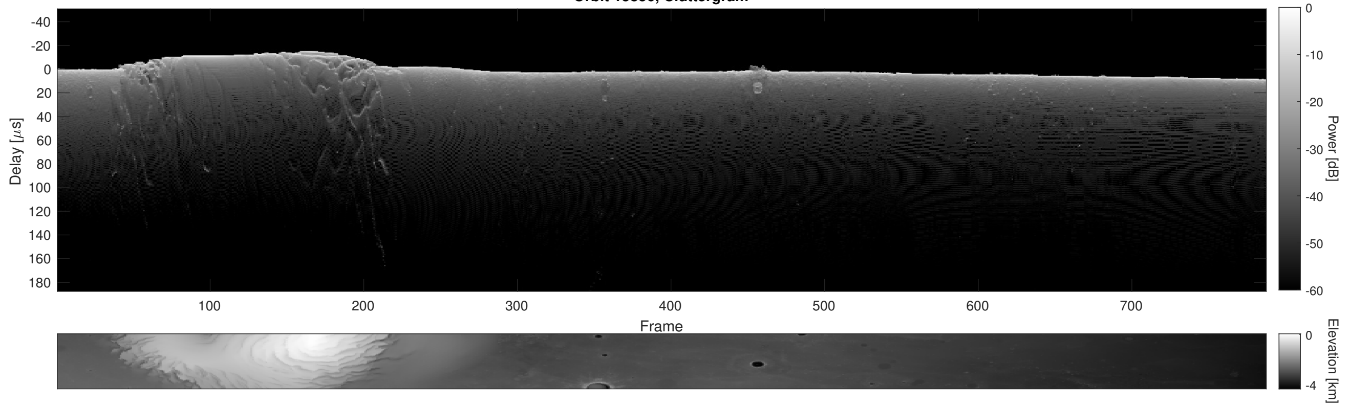
Orbit 15856, Cluttergram
