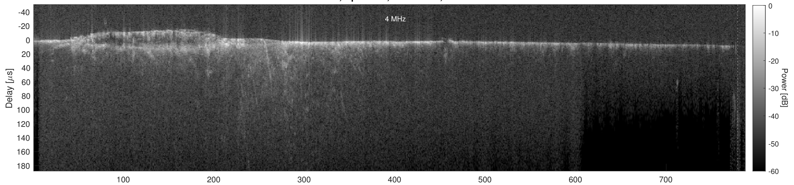
Orbit 15856, Cluttergram
