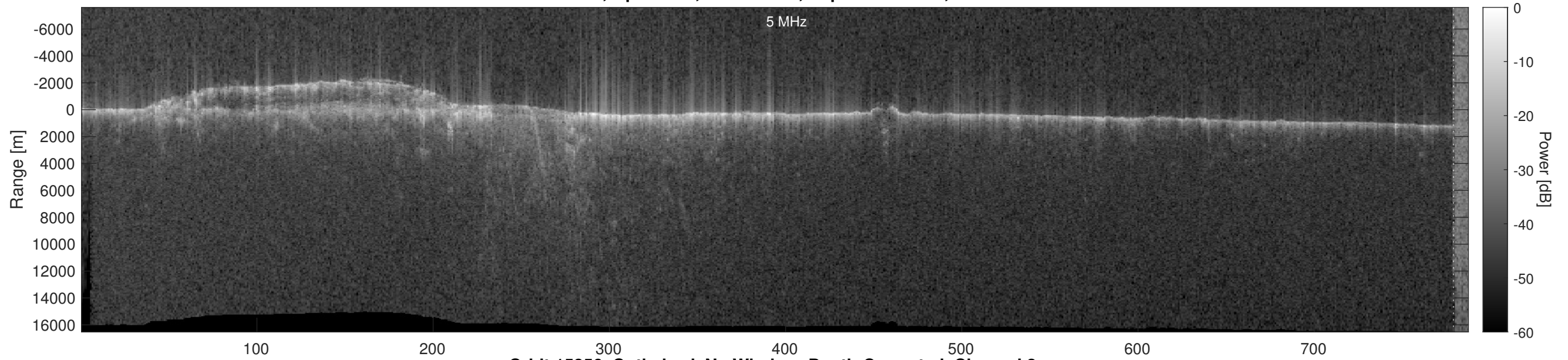
Orbit 15856, Optimized, No Window, Depth-Corrected, Channel 2
