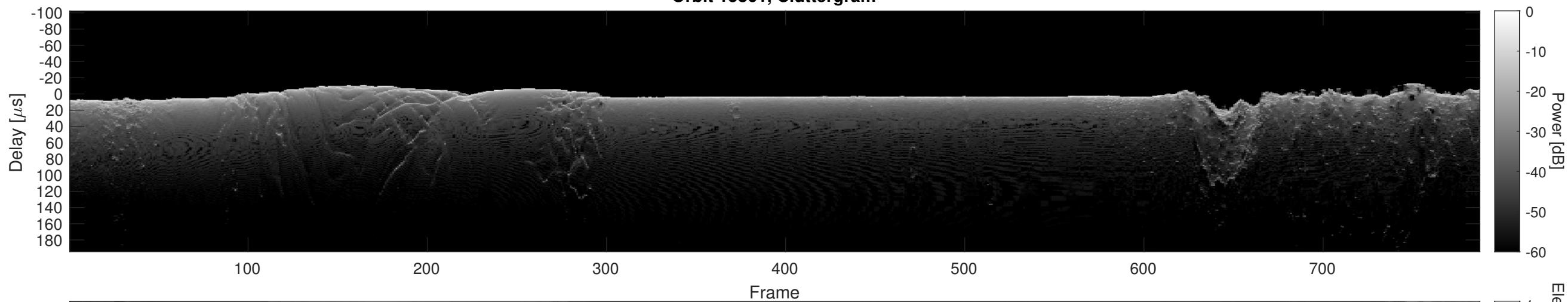
Orbit 15861, Cluttergram
