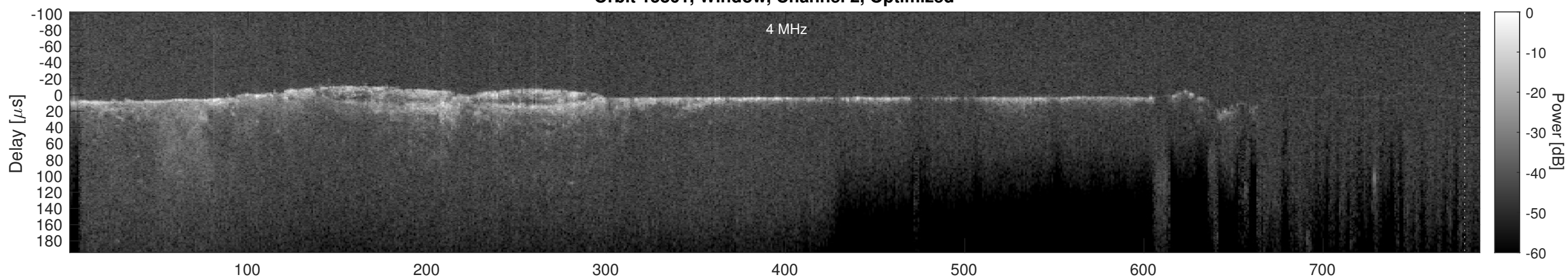
Orbit 15861, Cluttergram
