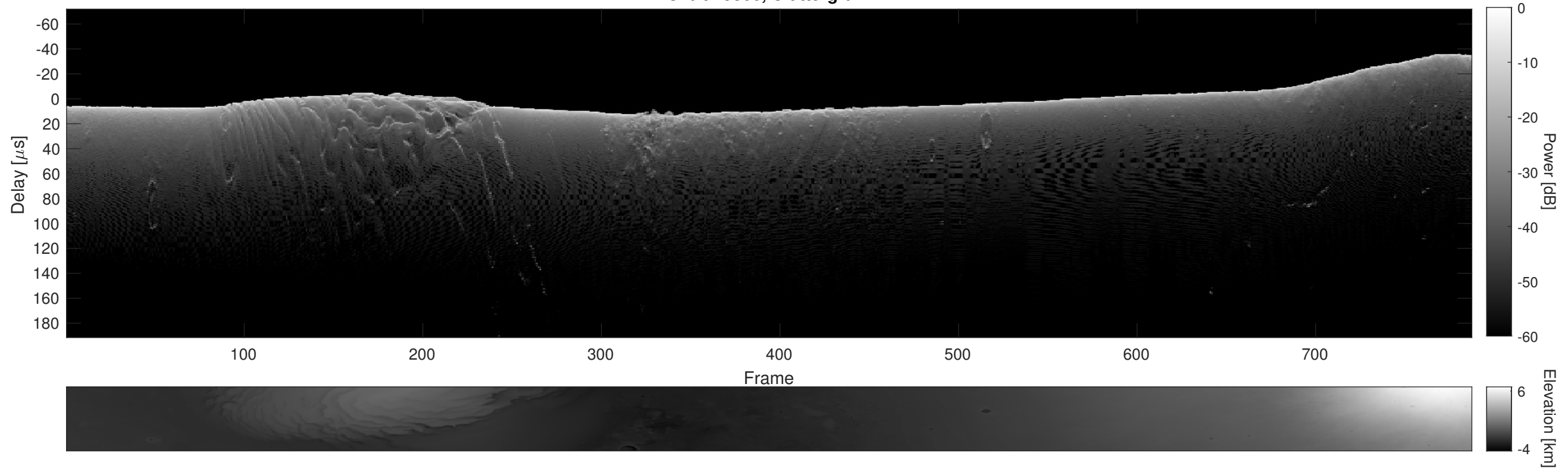
Orbit 15866, Cluttergram
