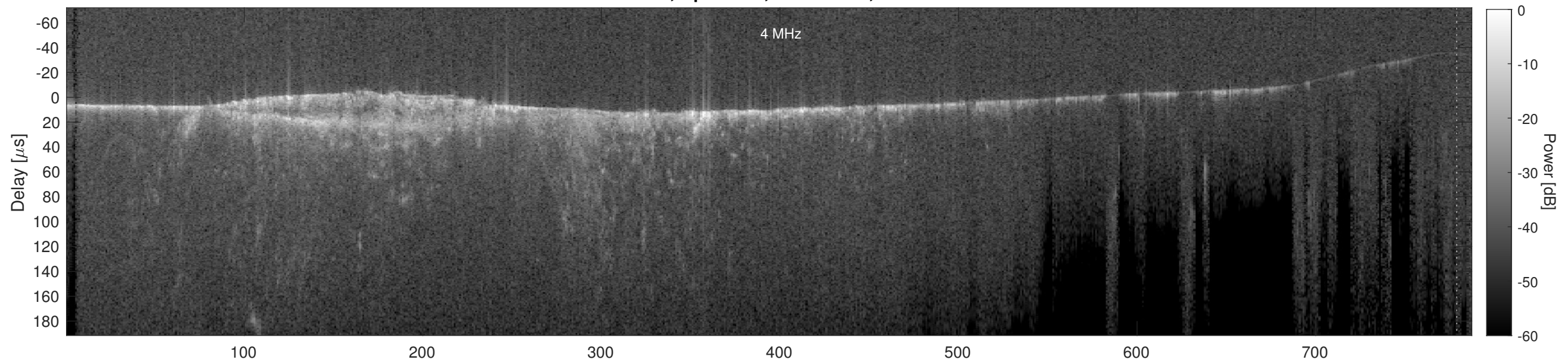
Orbit 15866, Cluttergram
