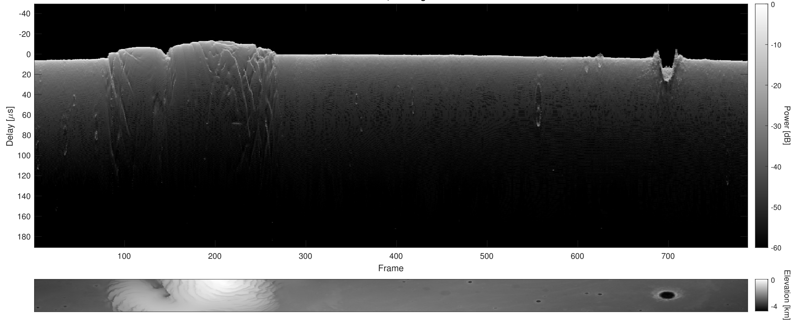
Orbit 15874, Cluttergram
