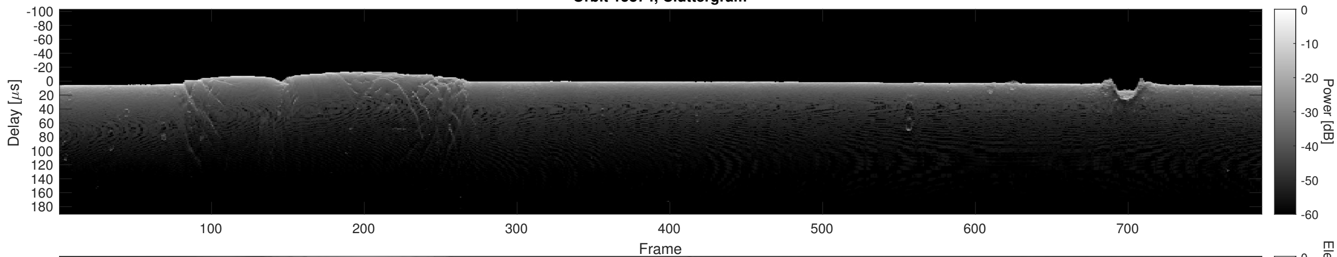
Orbit 15874, Cluttergram
