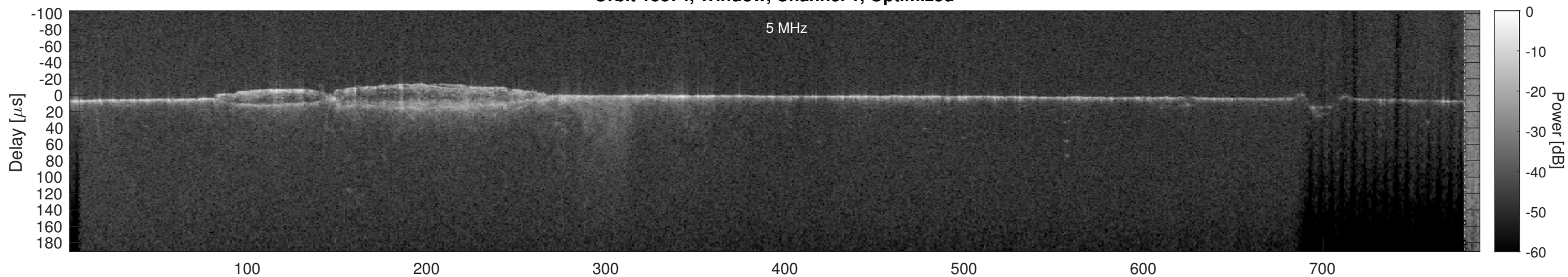
Orbit 15874, Cluttergram
