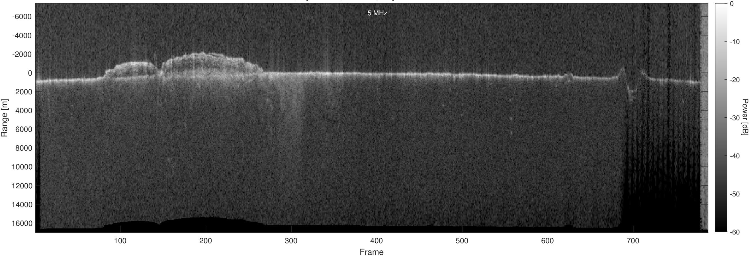
Orbit 15874, Optimized, Window, Depth-Corrected, Channel 2
