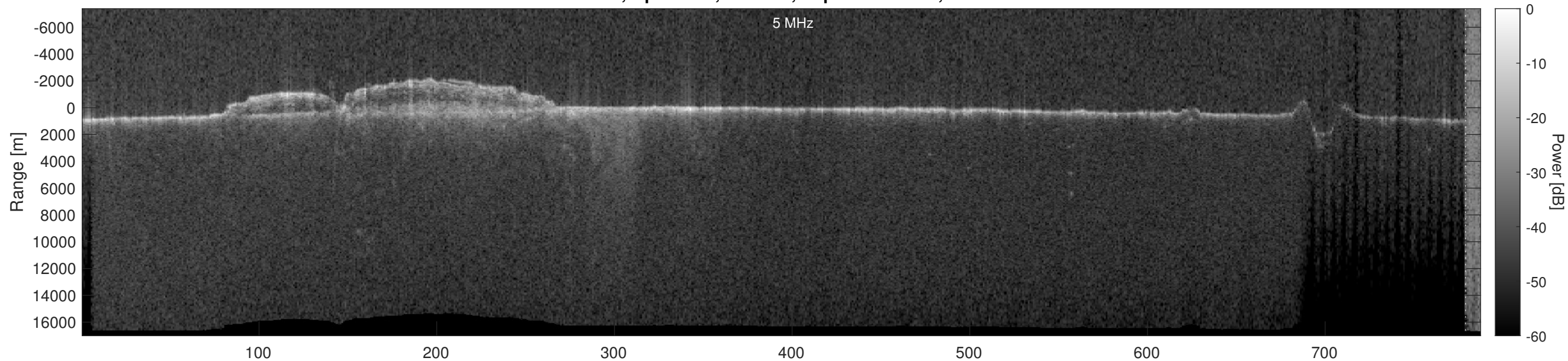
Orbit 15874, Optimized, Window, Depth-Corrected, Channel 2
