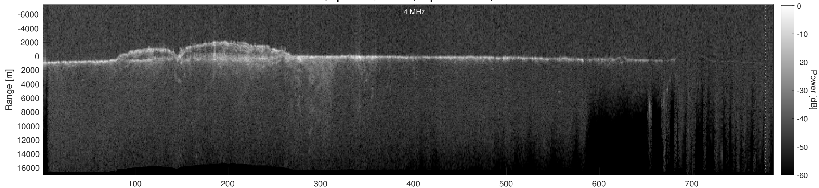
Orbit 15874, Depth-Corrected Cluttergram
