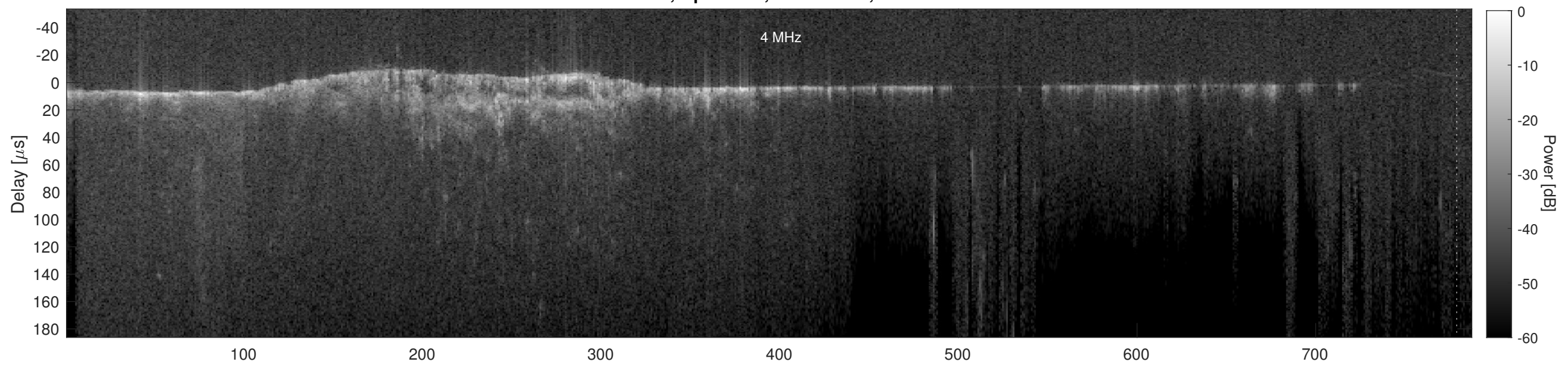
Orbit 15875, Cluttergram
