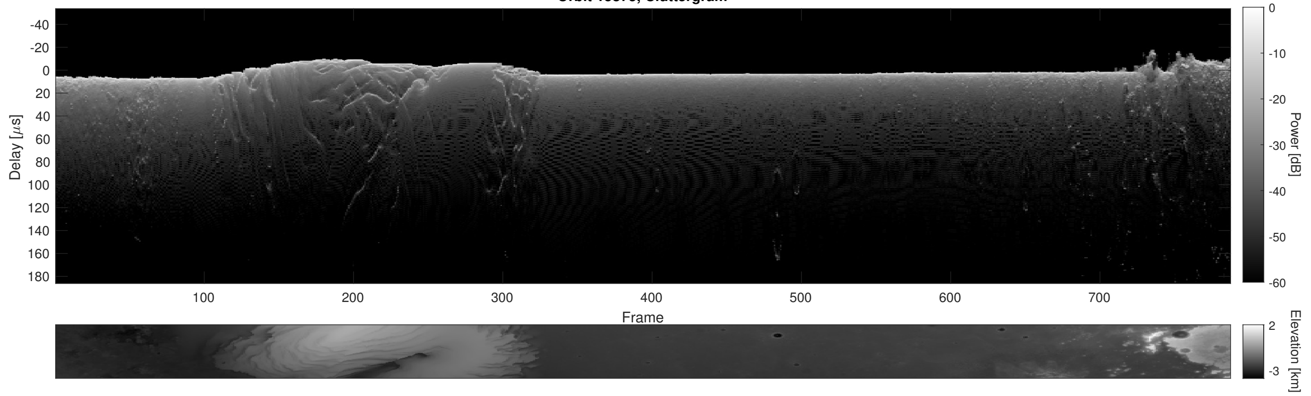
Orbit 15875, Cluttergram
