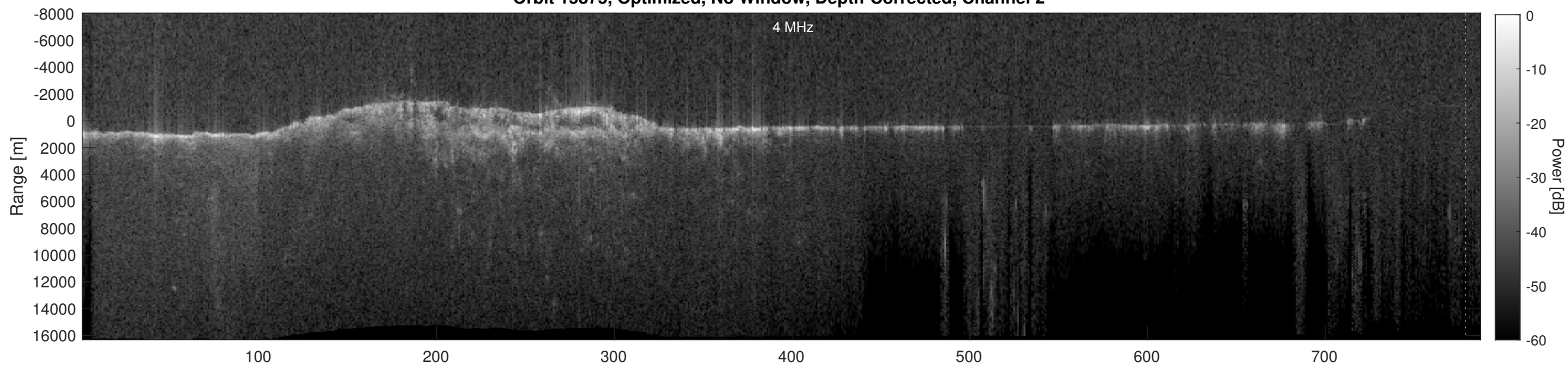
Orbit 15875, Depth-Corrected Cluttergram
